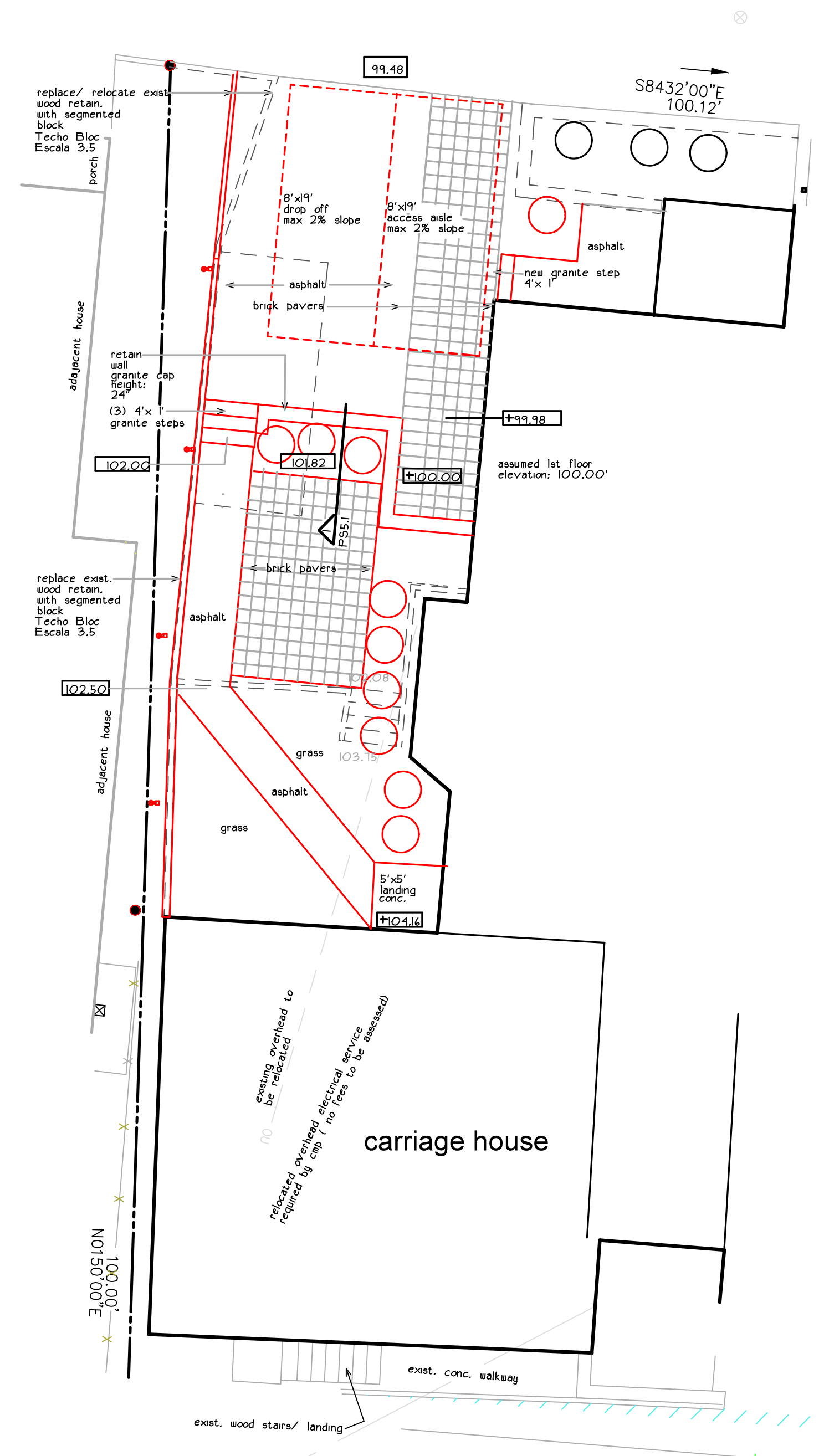
proposed partial site plan area of change 1/8"=1'-0" 0 4 8
