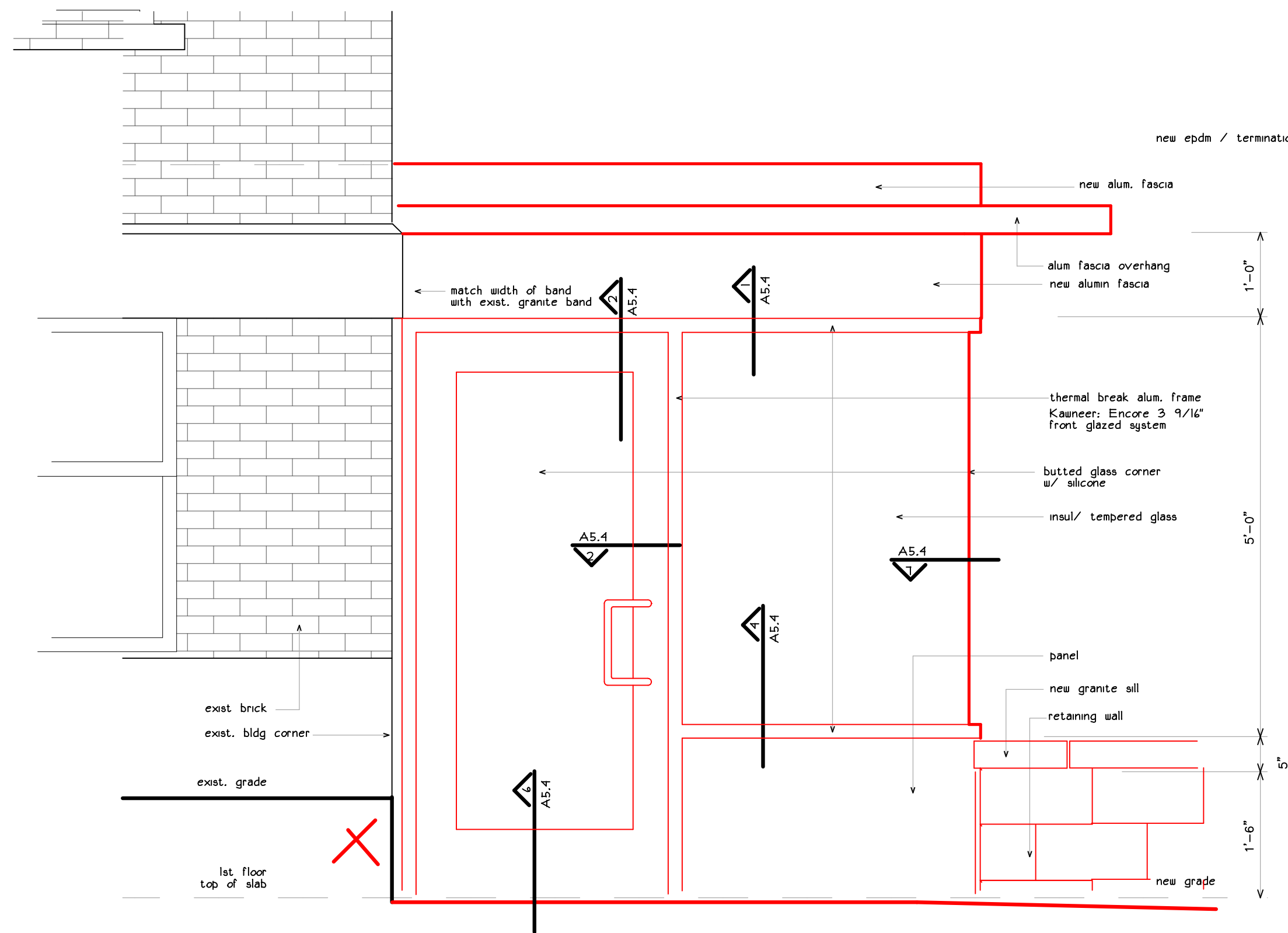
front vestibule elevation
