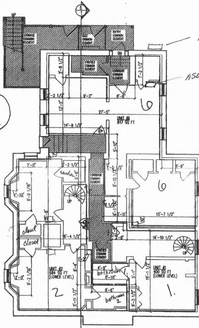
1 | LOWER LEVEL FLOOR PLAN SCALE: 1/8"=1'-0"
