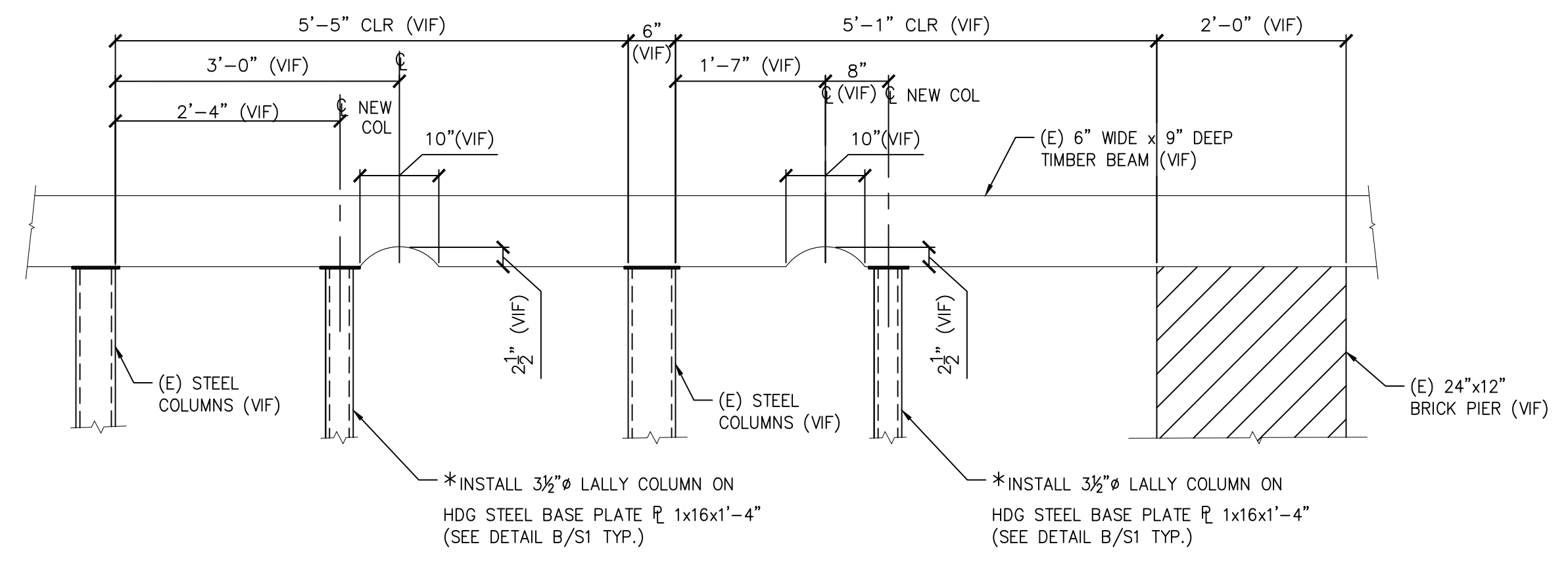
SECTION 5 RE-SUPPORT OF EXISTING COMPROMISED FIRST FLOOR BEAM 3/4" = 1'-0"
