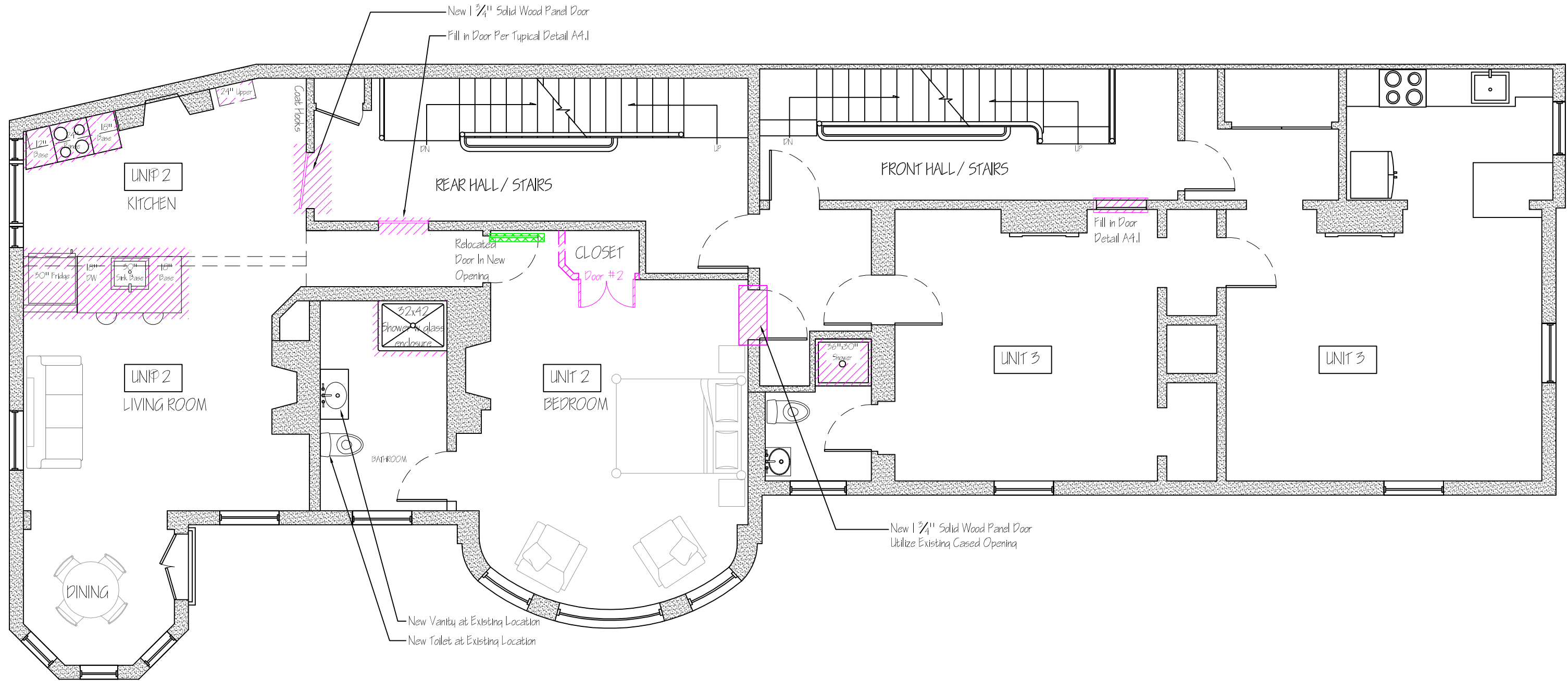
1 SECOND FLOOR PLAN: Unit 2 Remodel SCALE: 3/16" = 1'-0"
