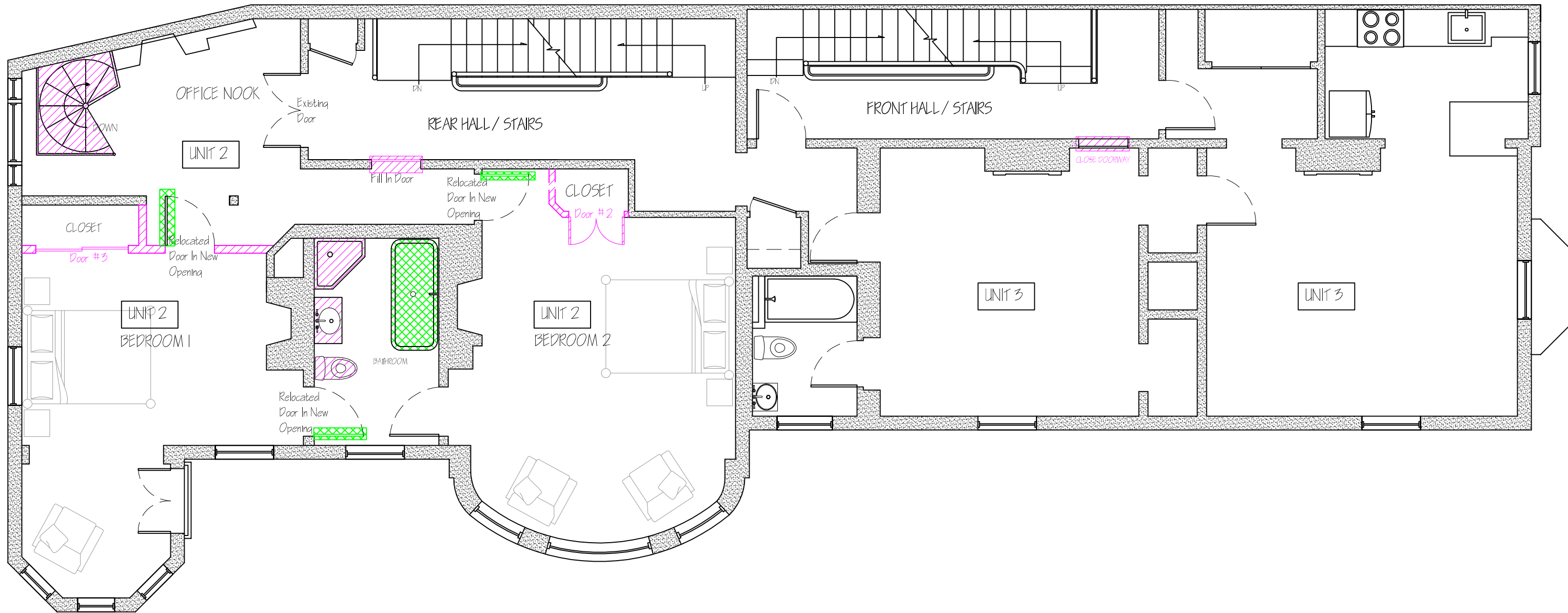
1 SECOND FLOOR PLAN: Unit 2 Remodel SCALE: 3/16" = 1'-0"
