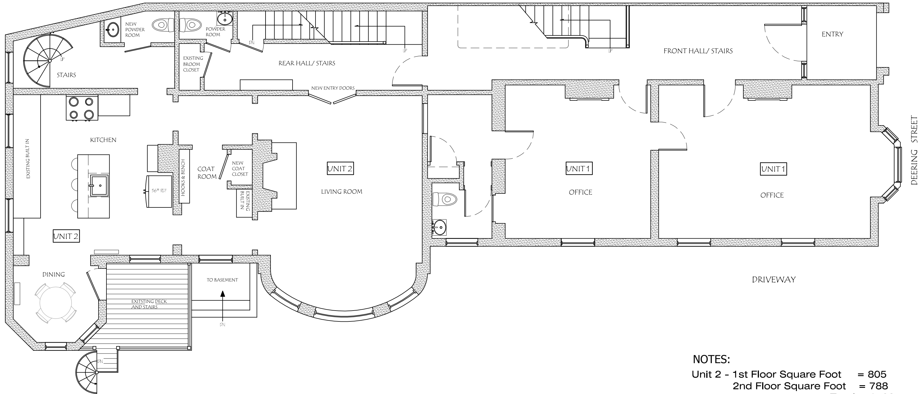
1 NEW FIRST FLOOR PLAN: UNIT 2 SCALE: 3/16" = 1'-0"
