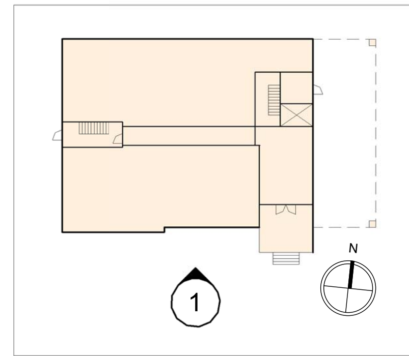
BUILDING B KEY PLAN
