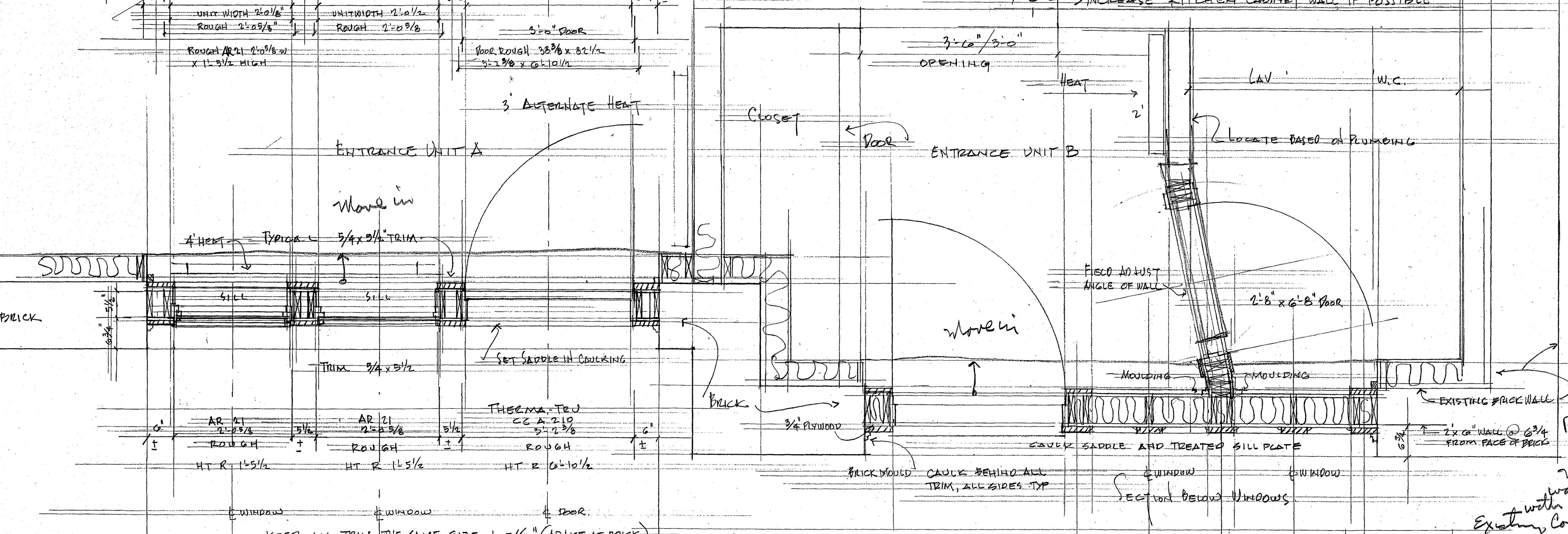
PLAN & ELEVATION UNIT A ENTRANCE 1"=1'-0" SEE UNIT B PLAN SECTION BELOW WINDOWS KEEP ALL TRIM THE SAME SIZE ± 5/16" (ADJUST AT BRICK) 9'-0" ± EXISTING BRICK FIELD MEASURE & FIELD ADJUST
