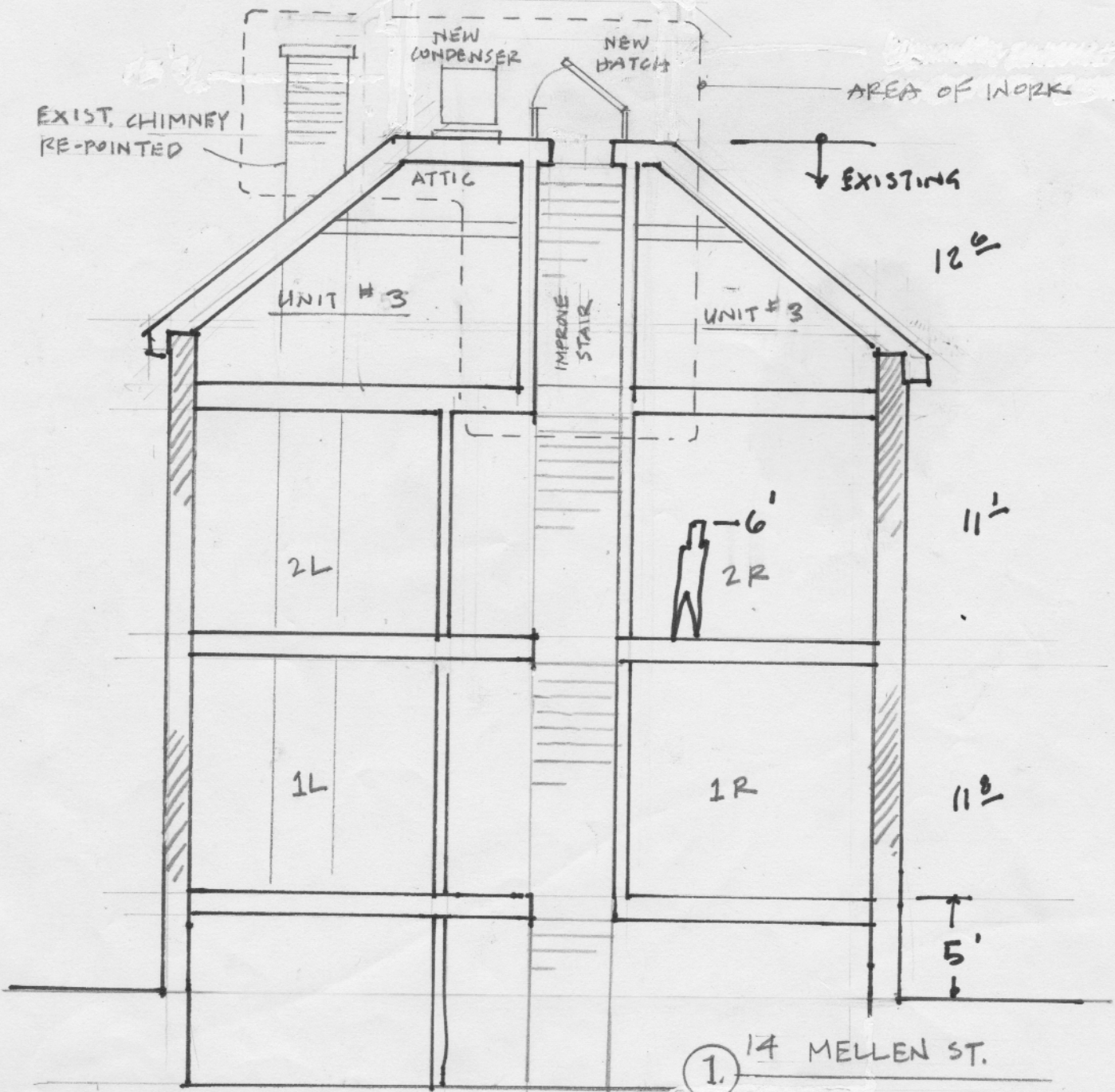
SCHMATIC SECTION C 14 MELLEN ST. 8.14.14 1/8" = 1'-0"
