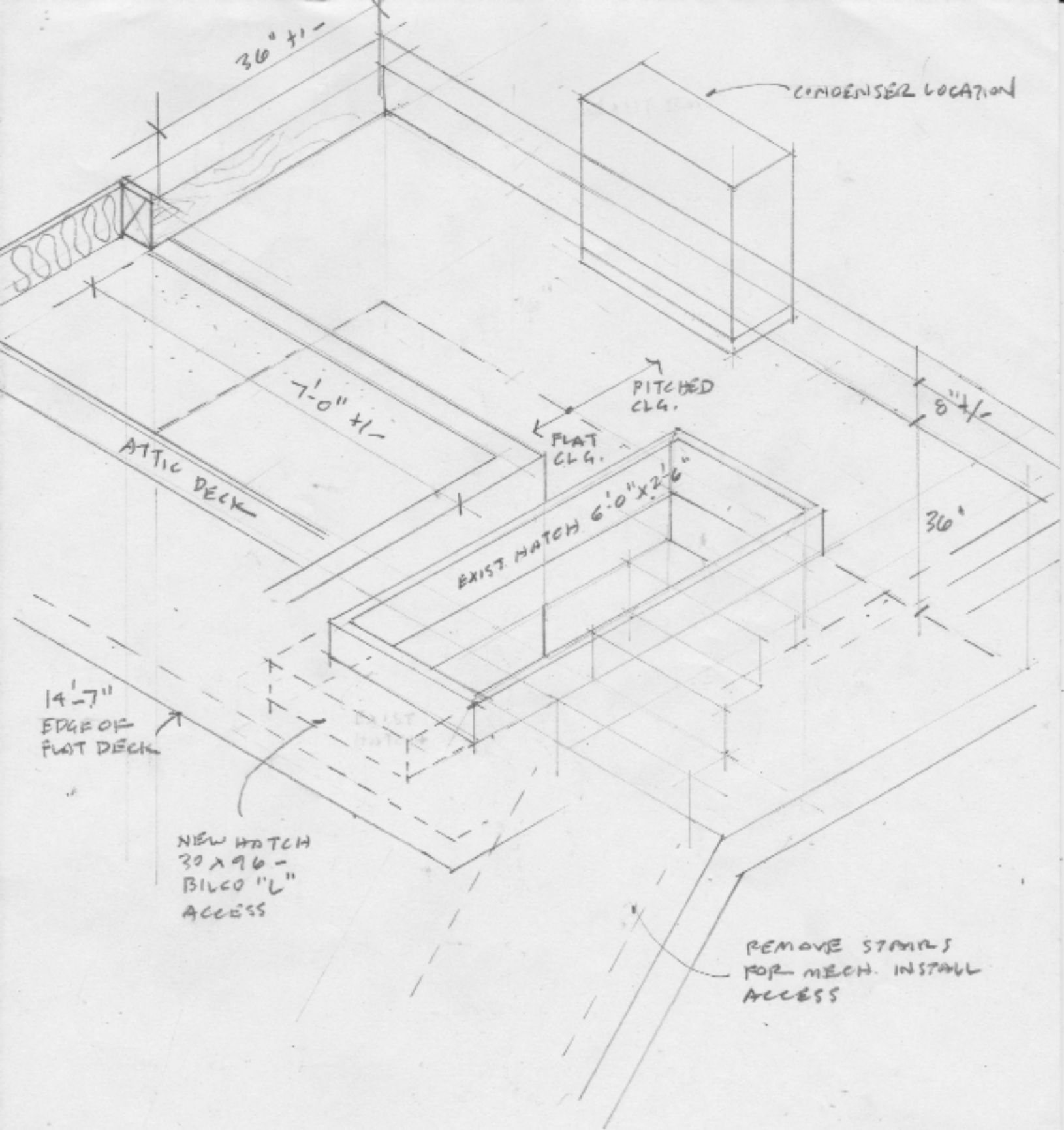
④ ATTIC SKETCH - 14 MELLEN ST. 1/2" = 1'-0" 10.10.14 WHIPPLE CALENDER ARCH.
