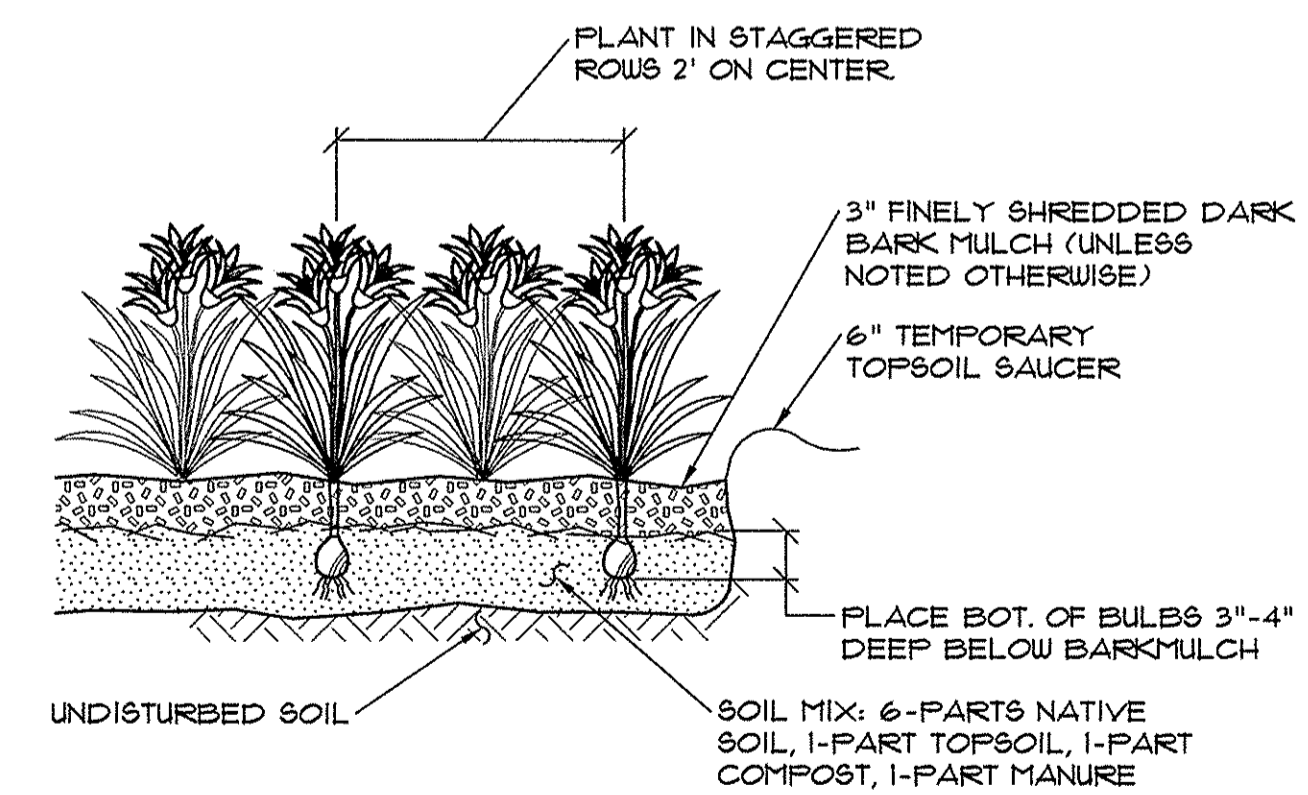
1 DAYLILY PLANTING DETAIL NOT TO SCALE
