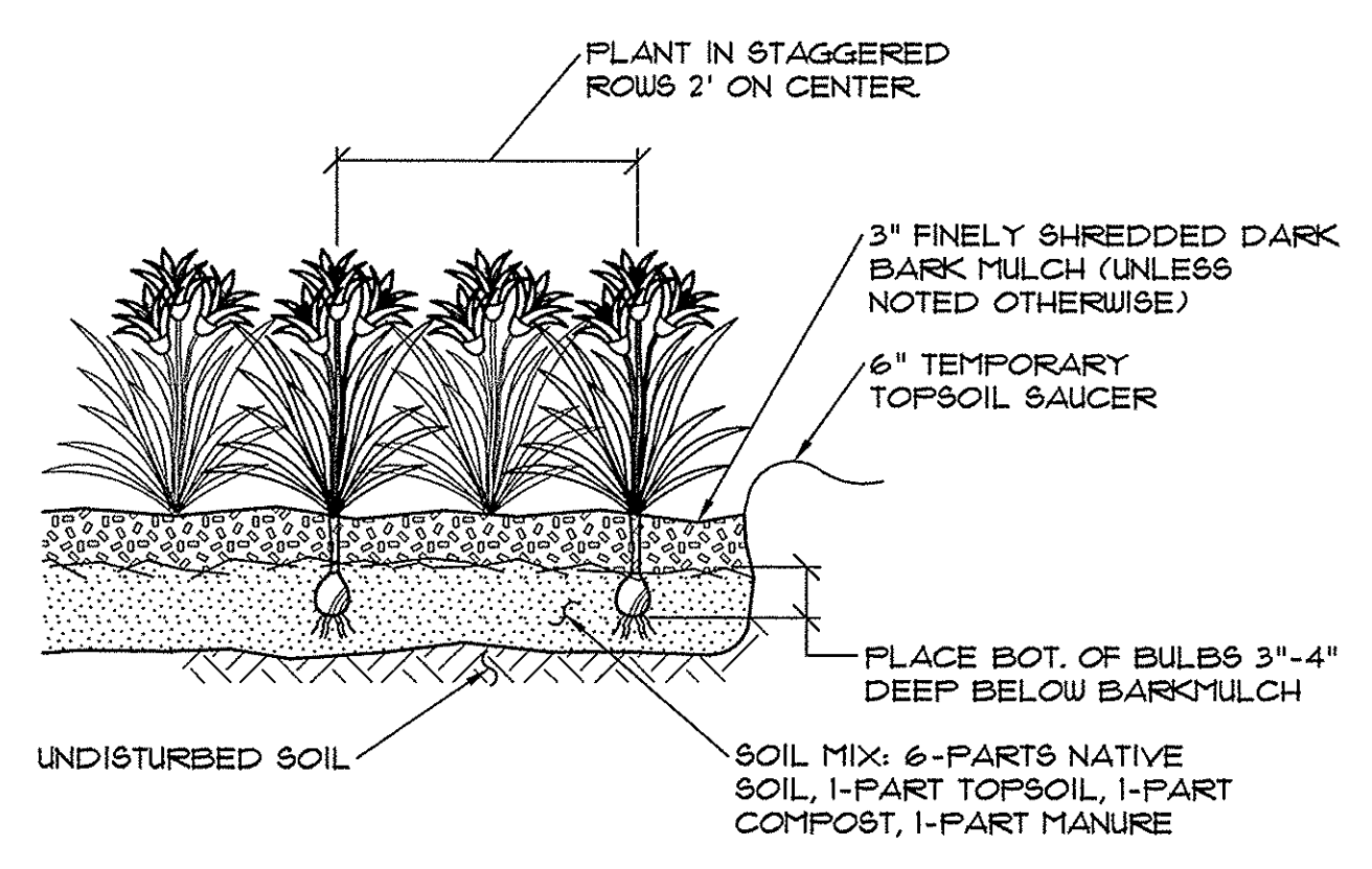
1 DAYLILY PLANTING DETAIL NOT TO SCALE
