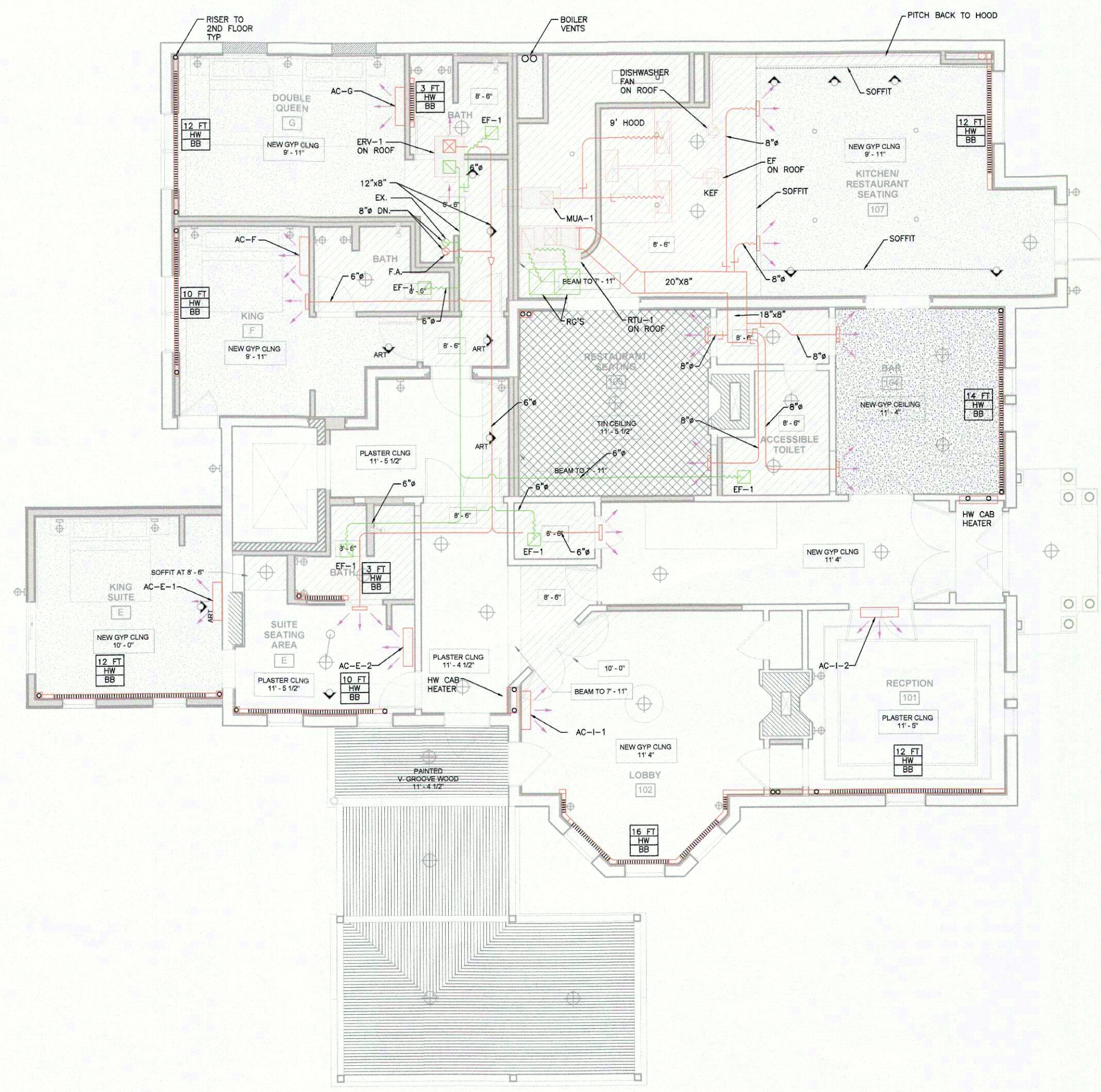
FIRST FLOOR - DUCTWORK SCALE: 3/16"=1'-0"
