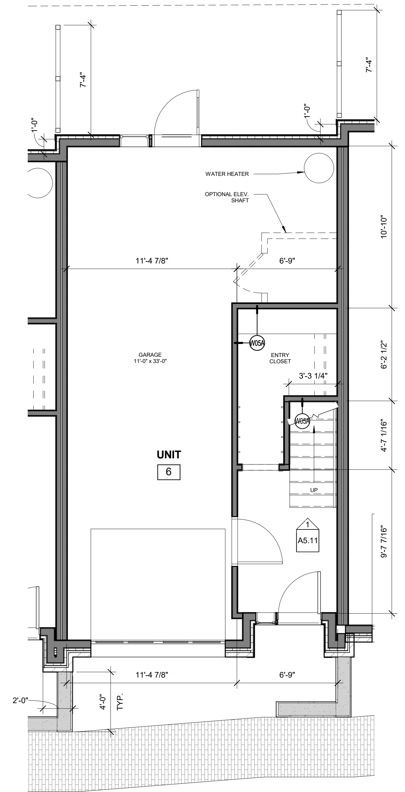
1 | 1ST FLOOR UNIT 6 1/4" = 1'-0"
