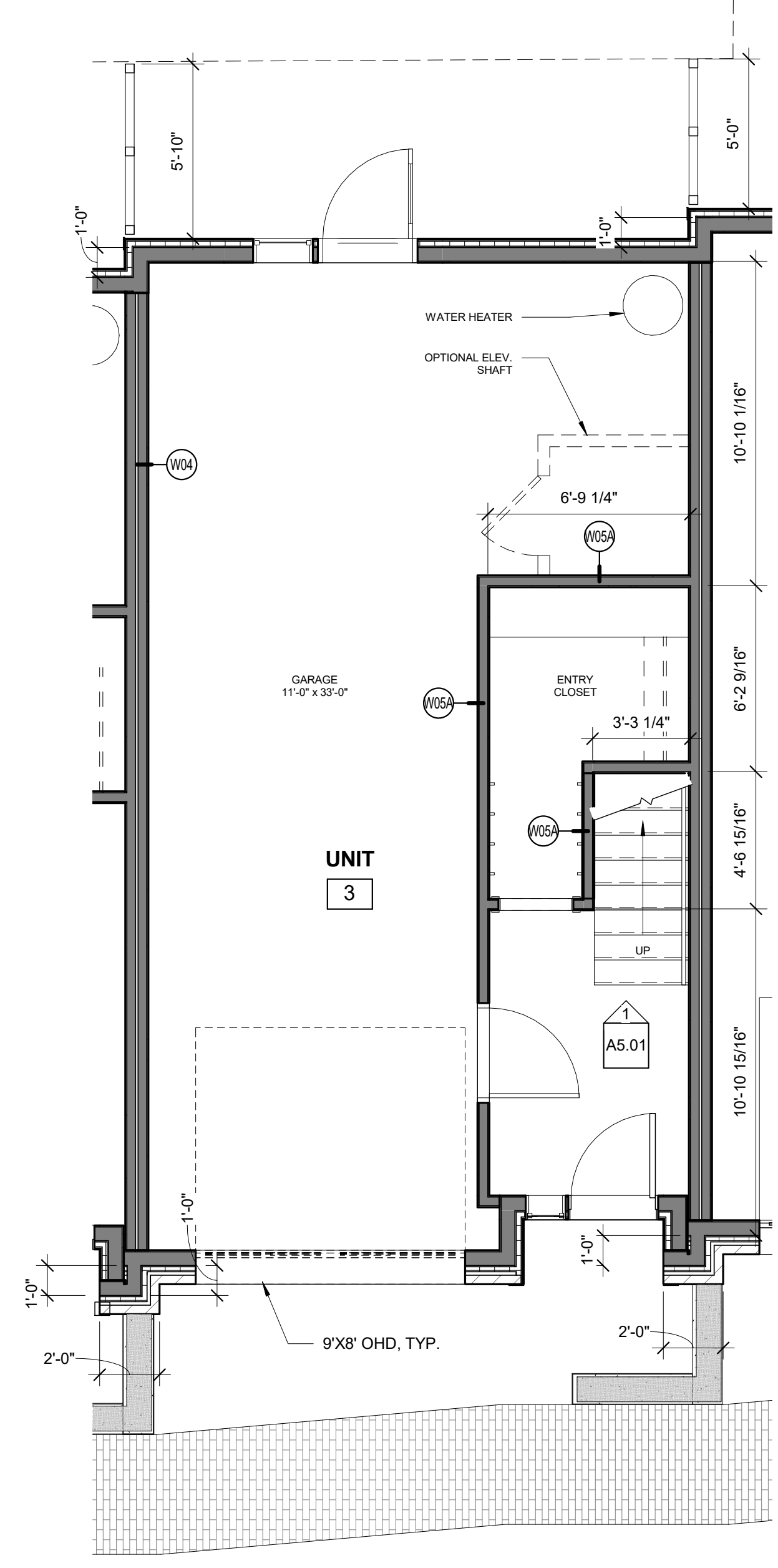
1 | 1ST FLOOR UNIT 3 1/4" = 1'-0"
