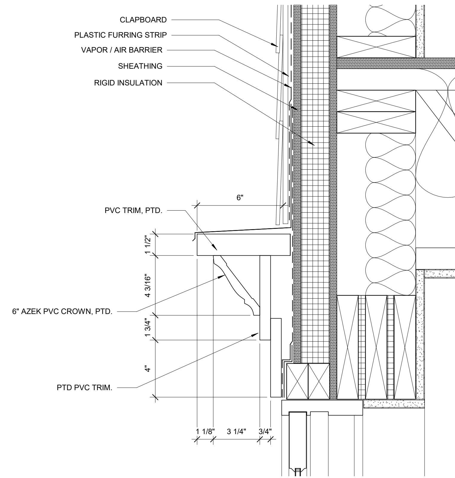
6 | CROWN ABOVE SLIDING DOOR DETAIL 3" = 1'-0"
