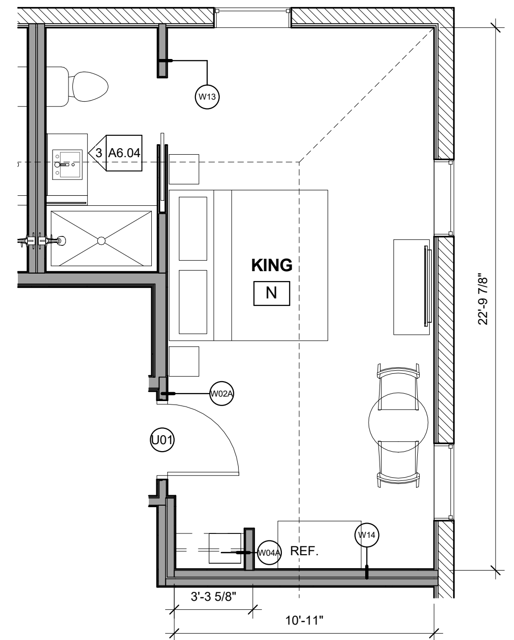
5 | 3RD FLOOR - KING - N 1/4" = 1'-0"
