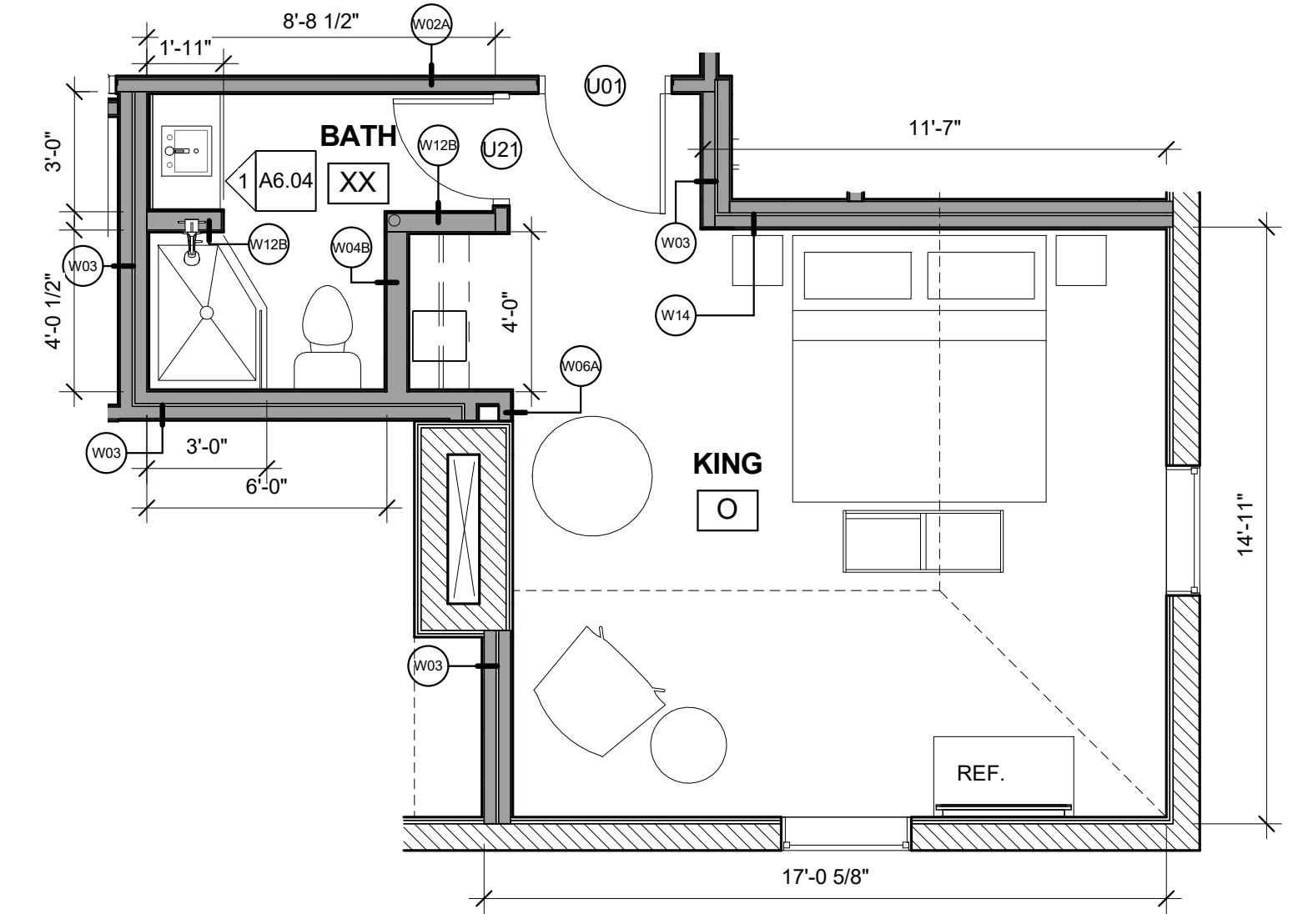
2 | 3RD FLOOR - KING - O 1/4" = 1'-0"
