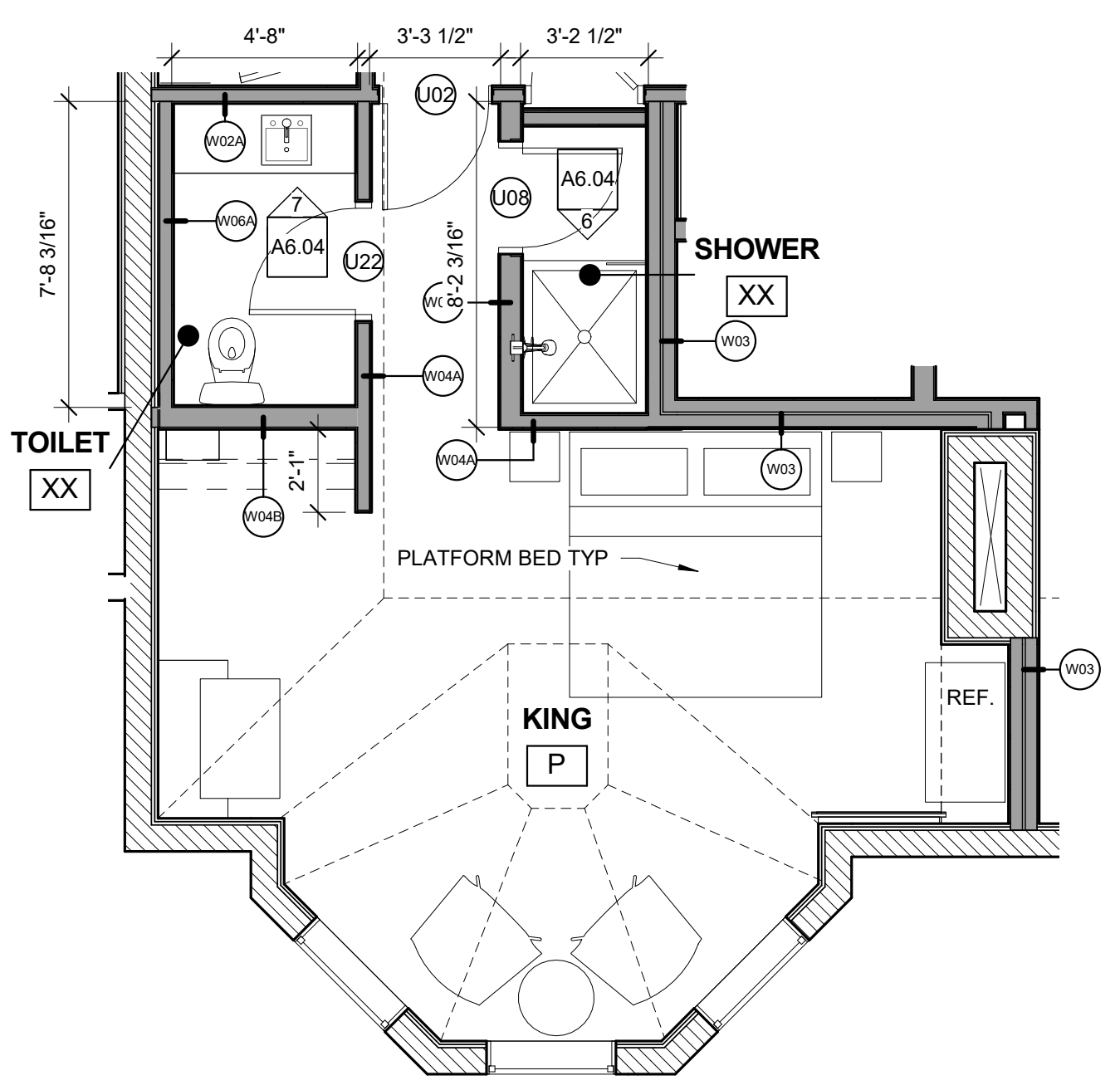
8 | 3RD FLOOR - KING - P 1/4" = 1'-0"
