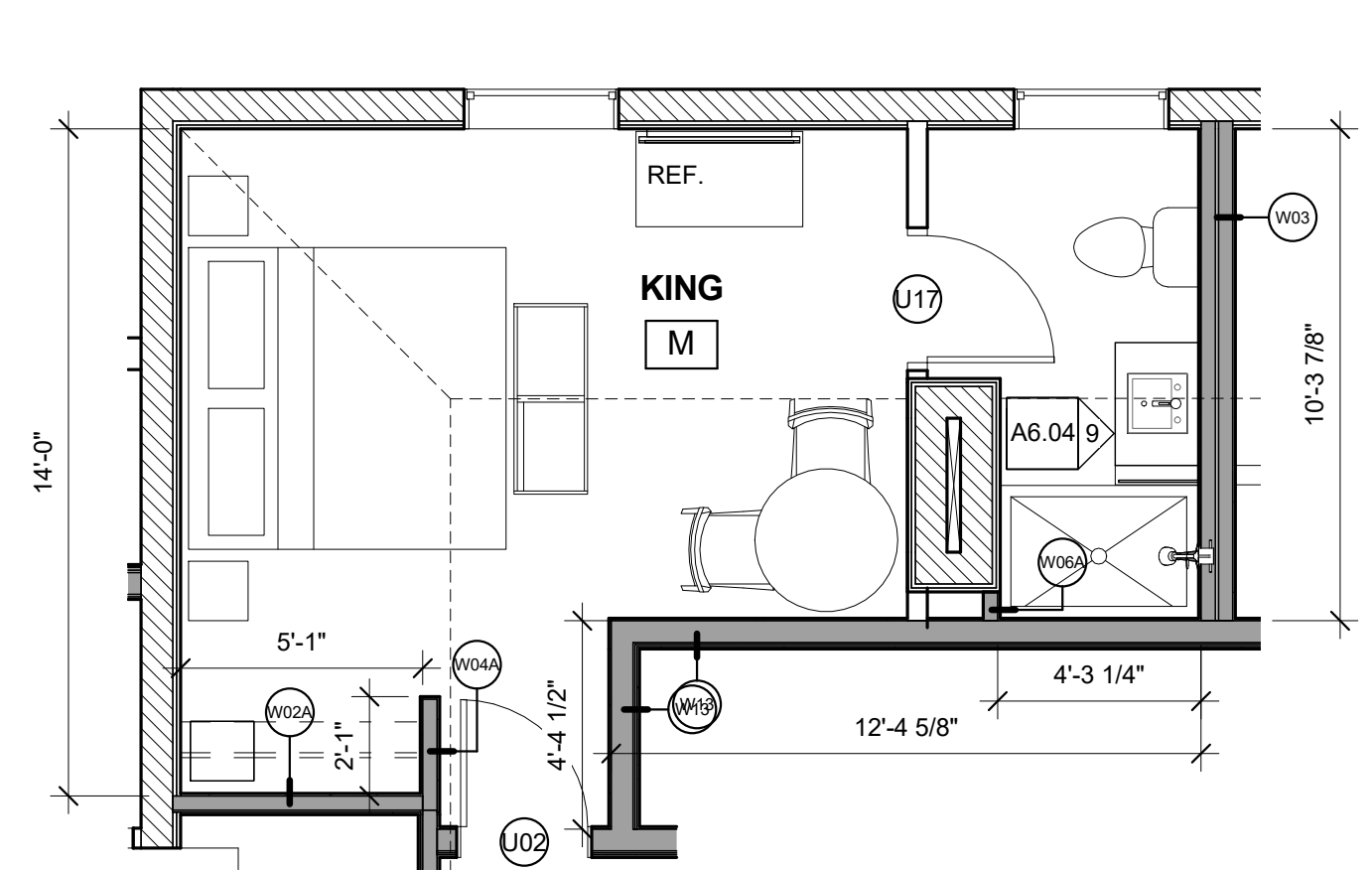
10 | 3RD FLOOR - KING - M 1/4" = 1'-0"
