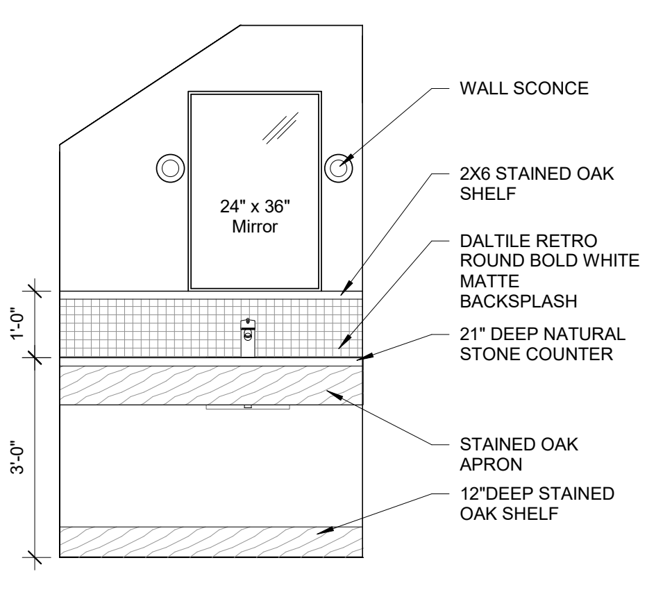
7 | KING P VANITY ELEVATION 1/2" = 1'-0"
