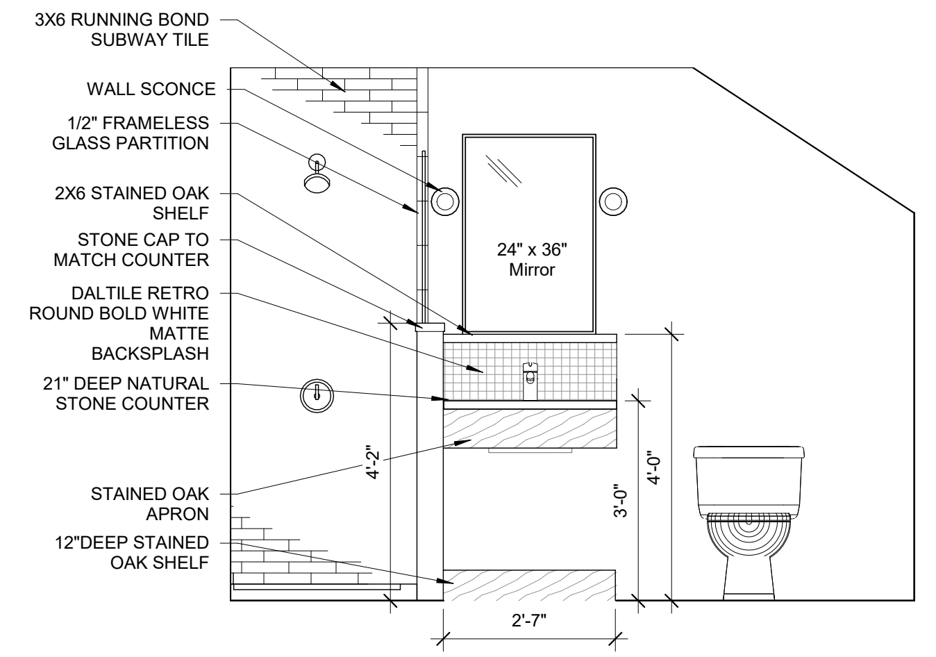
3 | KING M BATHROOM ELEVATION 1/2" = 1'-0"
