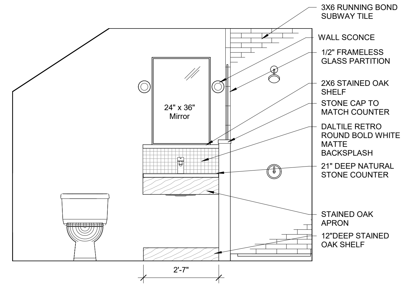
9 | KING M VANITY AND SHOWER ELEVATION 1/2" = 1'-0"
