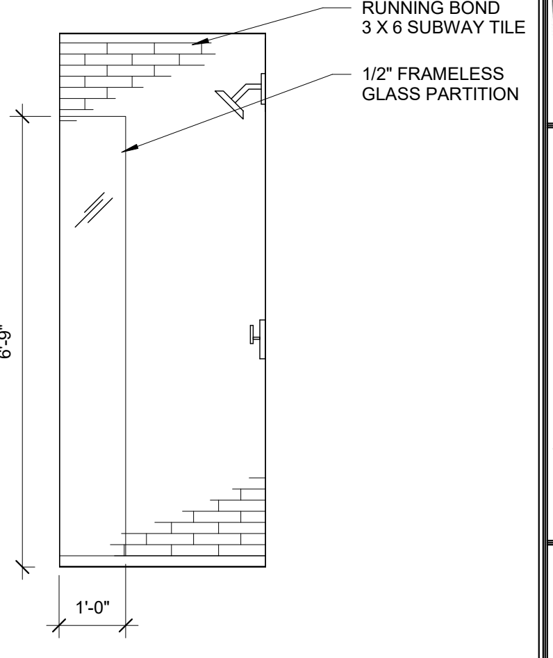
6 | KING P SHOWER 1/2" = 1'-0"
