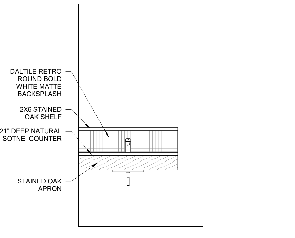
4 MASSAGE ROOM SINK ELEVATION 1/2" = 1'-0"
