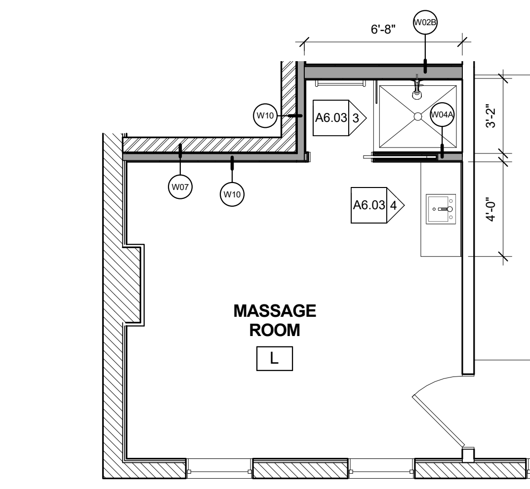
5 2ND FLOOR - MASSAGE ROOM - L 1/4" = 1'-0"
