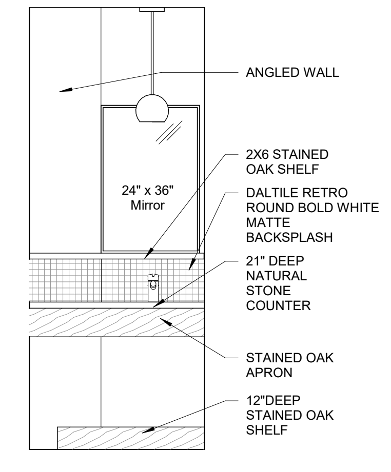
2 QUEEN J VANITY ELEVATION 1/2" = 1'-0"
