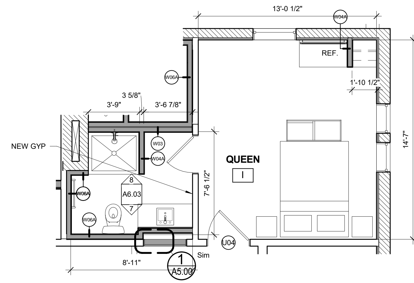
14 2ND FLOOR - QUEEN - I 1/4" = 1'-0"
