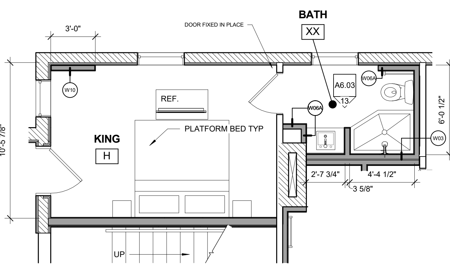
9 2ND FLOOR - KING - H 1/4" = 1'-0"
