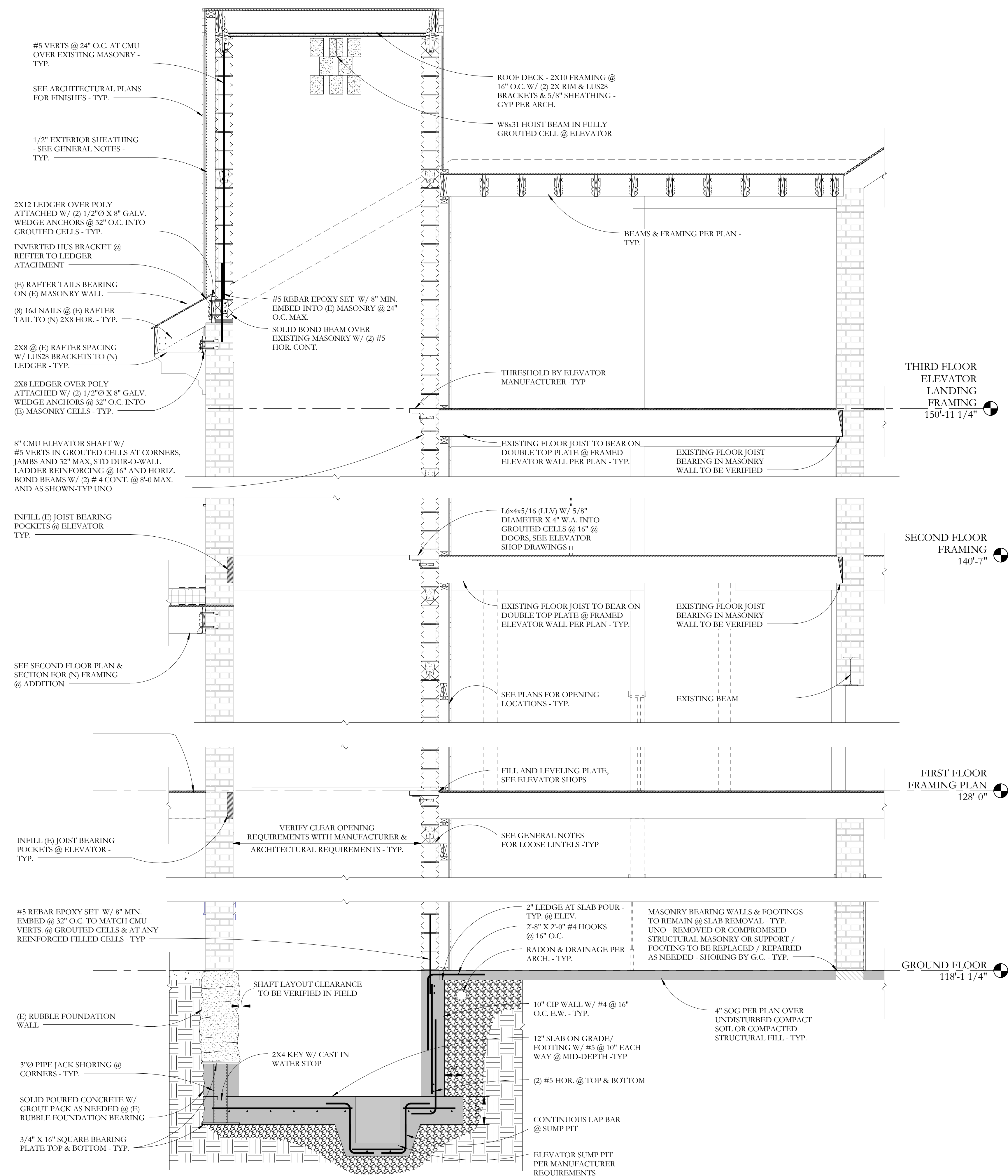
E ELEVATOR SECTION S2.1 1/2" = 1'-0"
