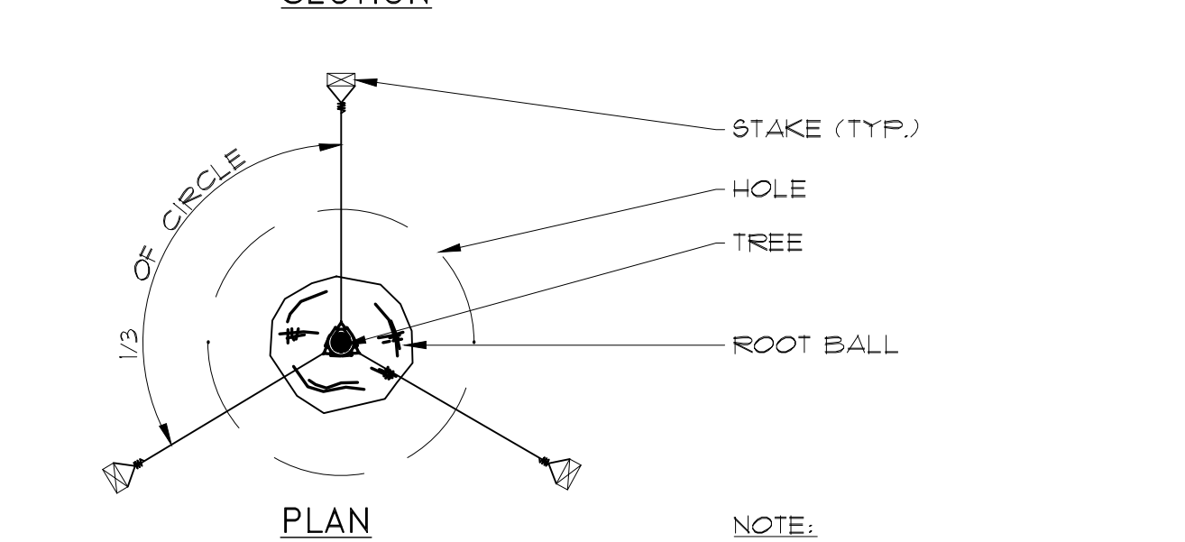
1 TREE PLANTING DETAIL NOT TO SCALE
