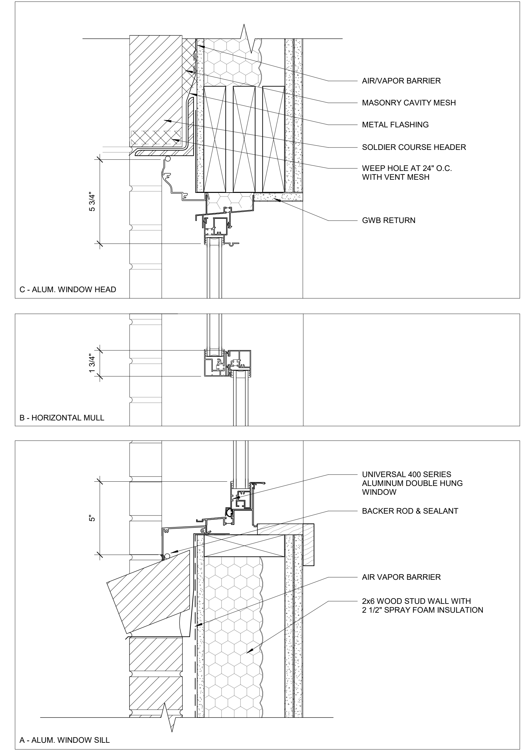
2 | NEW TYPE P WINDOW DETAIL 3" = 1'-0"
