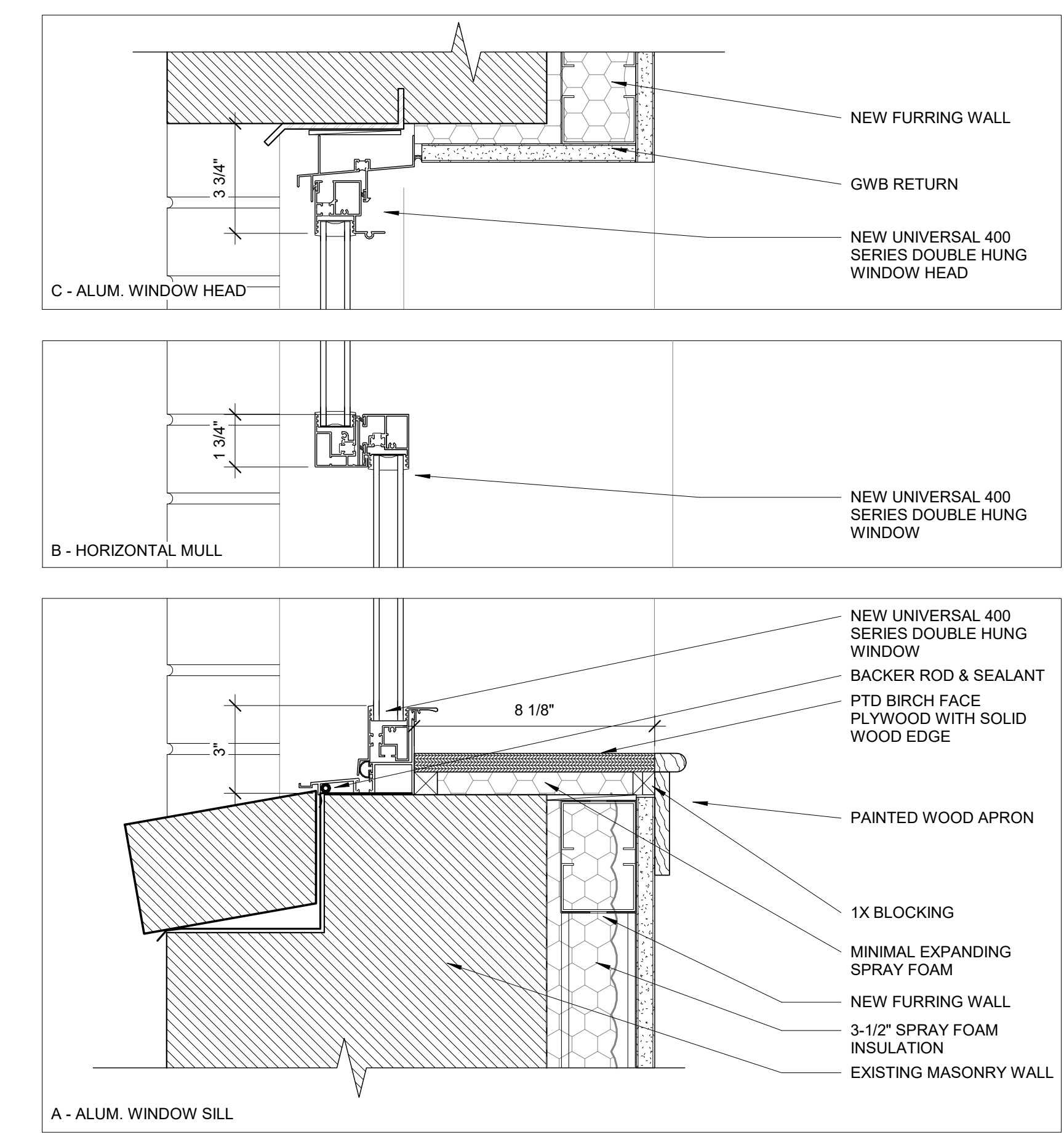
1 | NEW TYPE N WINDOW DETAILS 3" = 1'-0"
