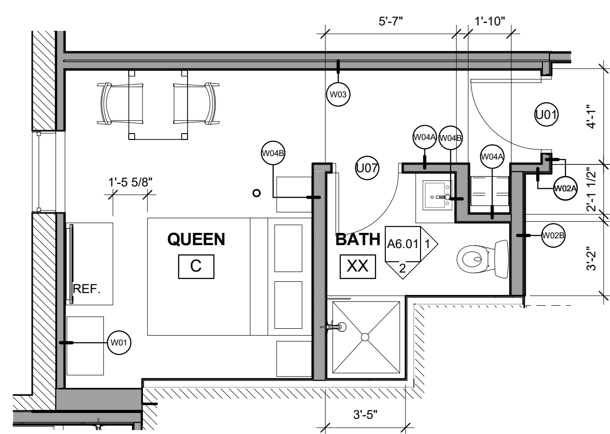
3 | GROUND FLOOR - QUEEN - C 1/4" = 1'-0"
