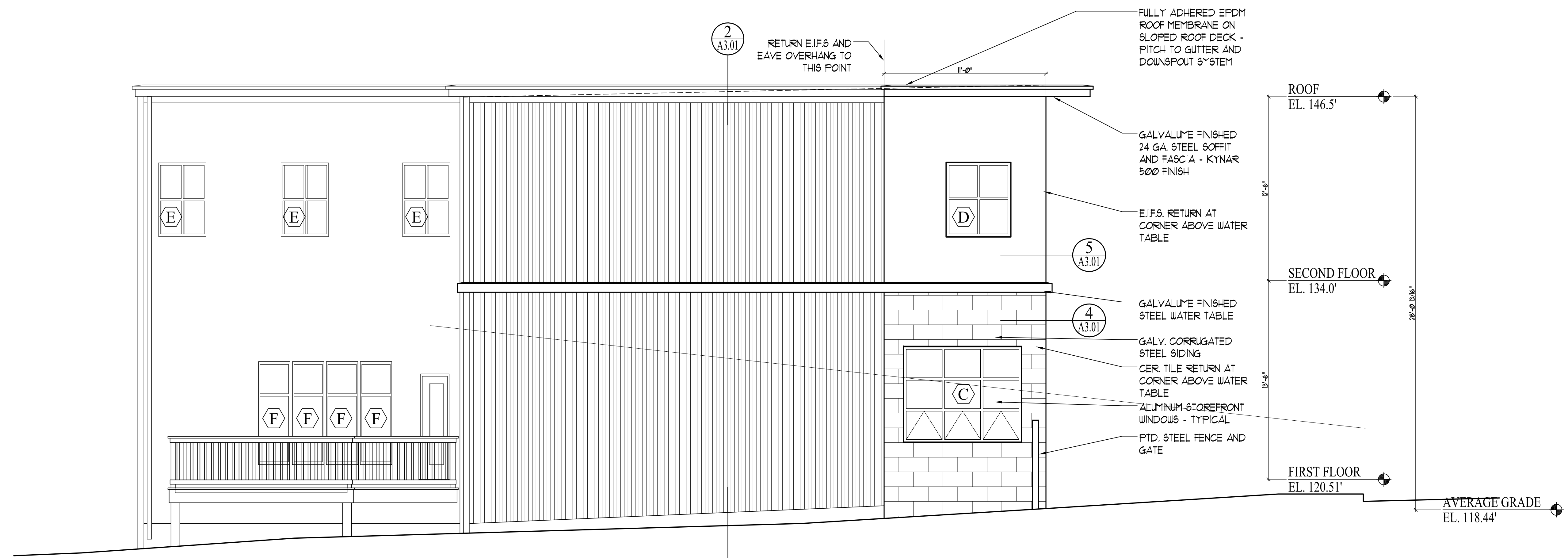
D WEST SIDE ELEVATION SCALE: 1/8"=1'-0"
