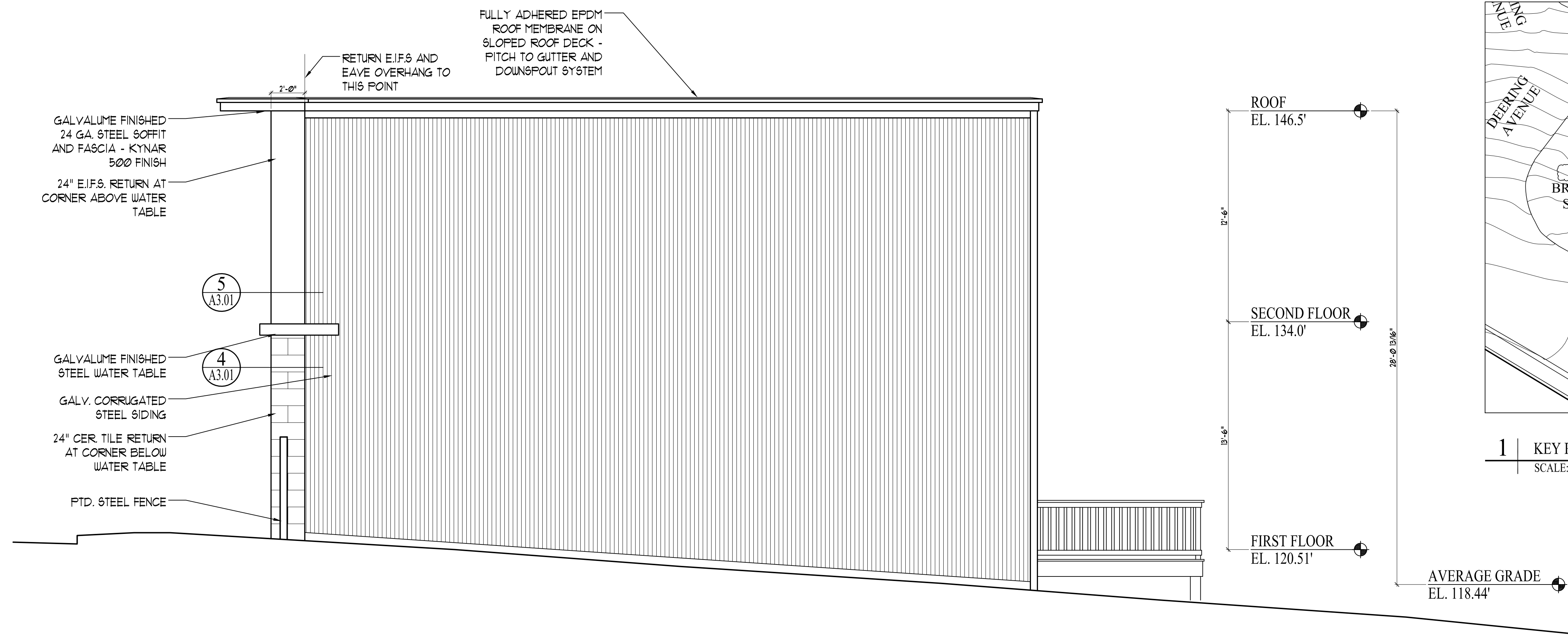
C EAST SIDE ELEVATION SCALE: 1/4"=1'-0"
