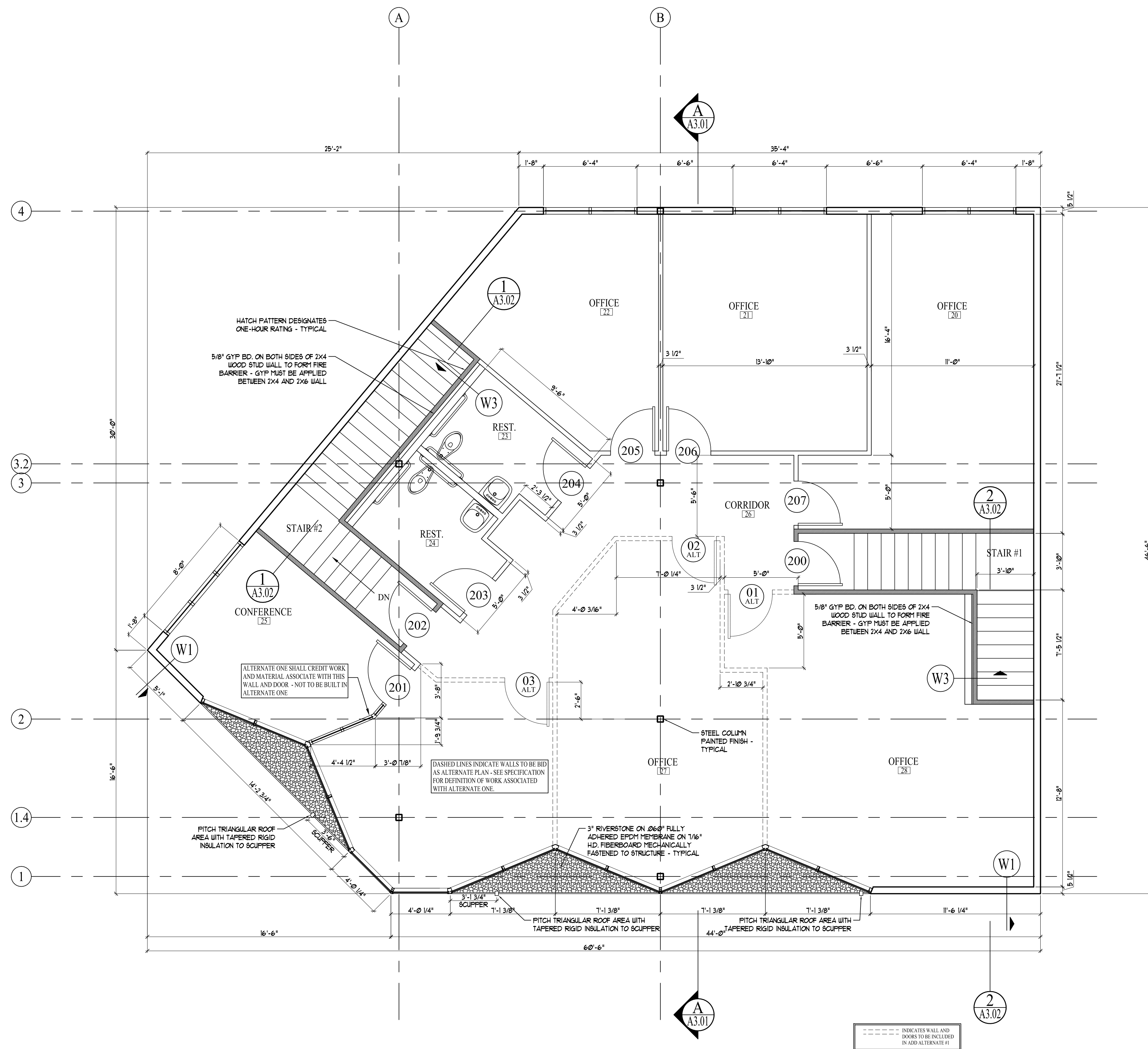
1 | BRAMHALL SQUARE FLOORPLAN- SECOND FLOOR SCALE: 1/4"=1'-0"
