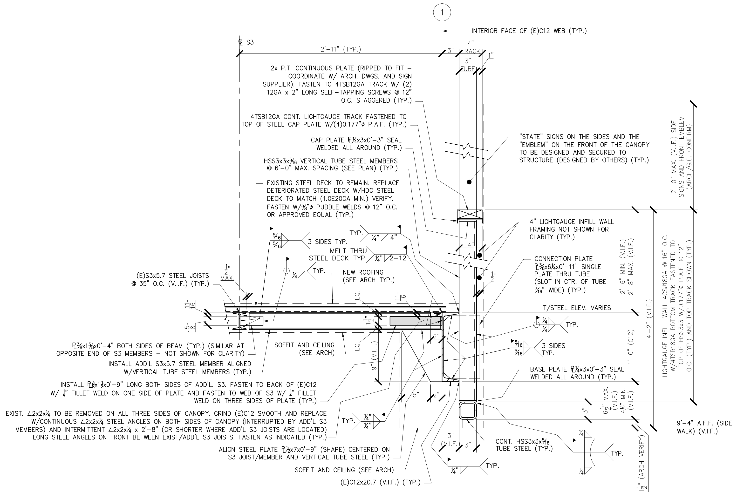
SECTION 1 1 1/2" = 1'-0"
