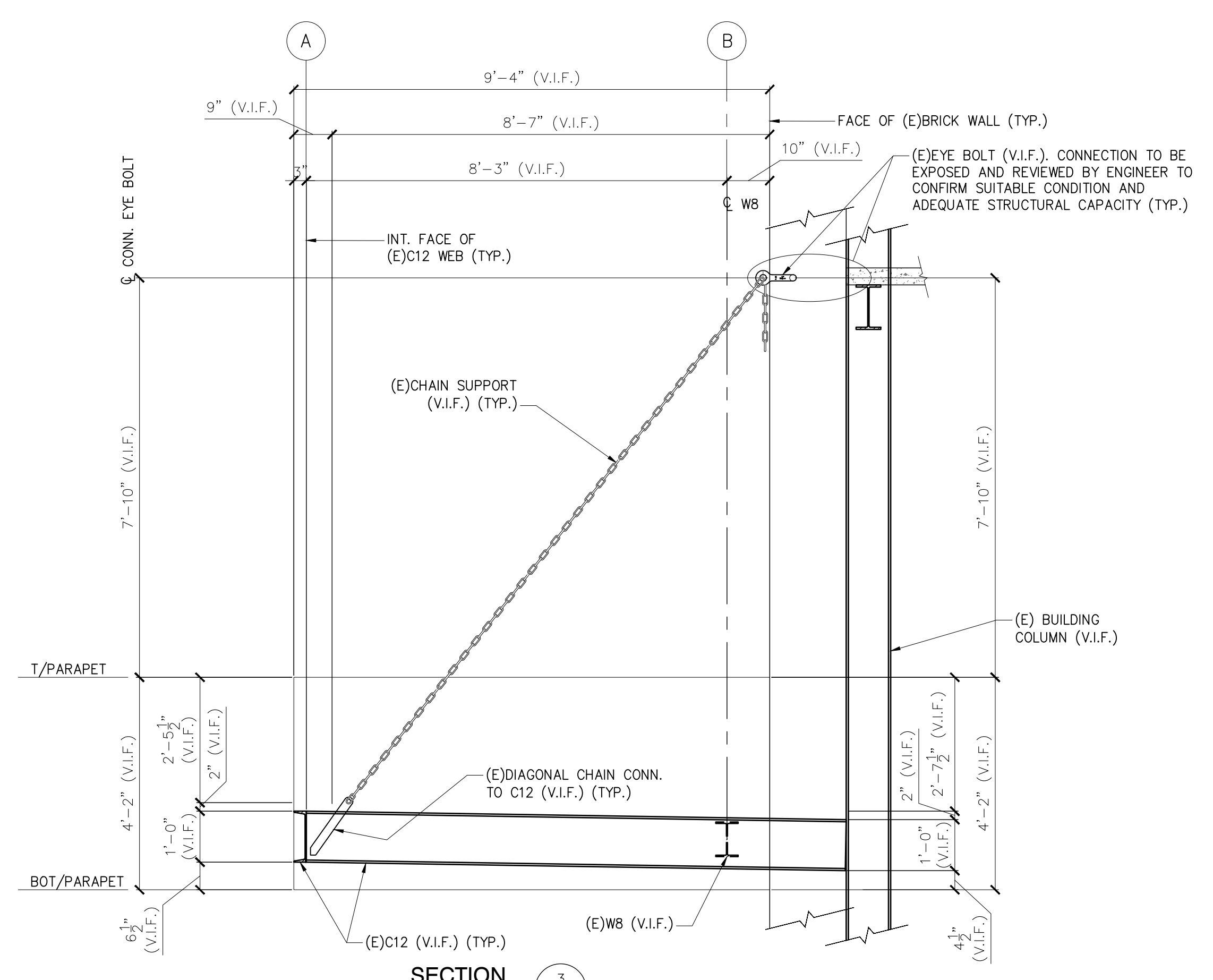
SECTION 3 1/2" = 1'-0"
