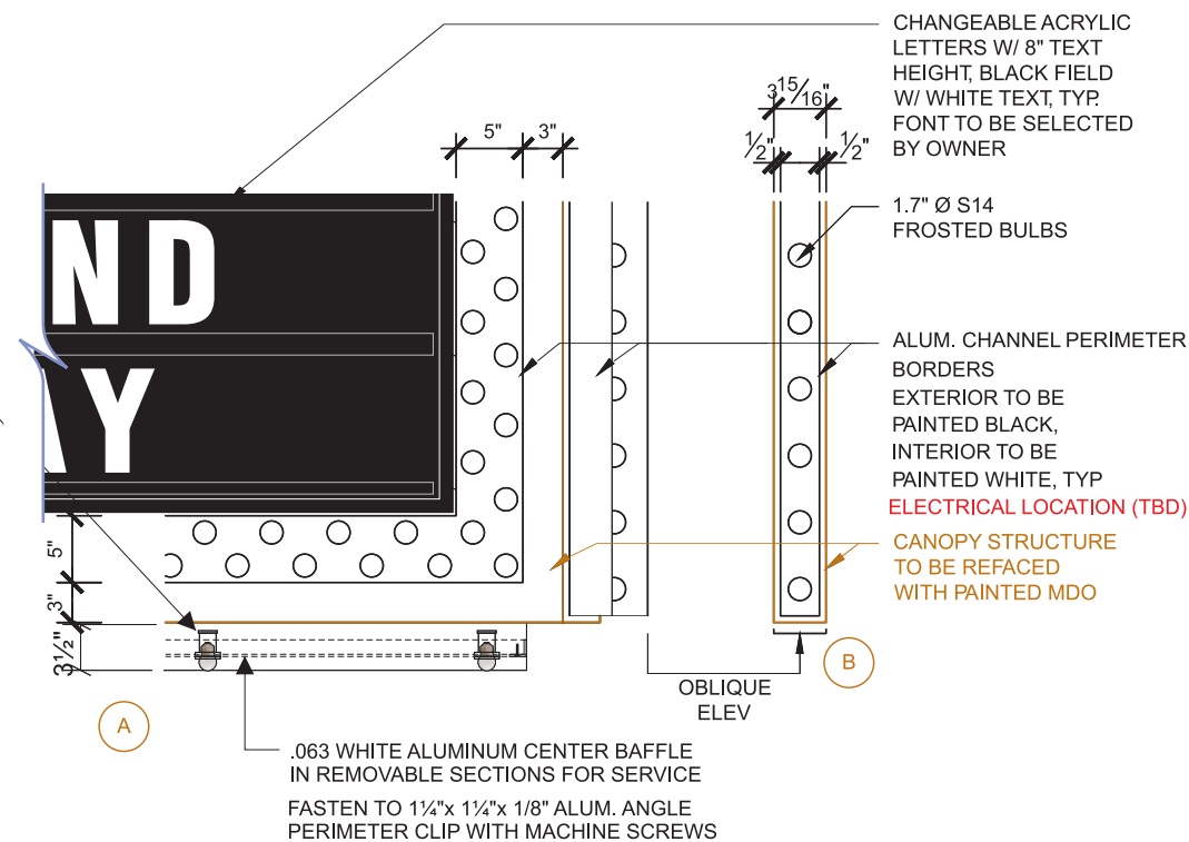
5 ELEVATION DETAIL SCALE: 3/4" = 1'-0"
