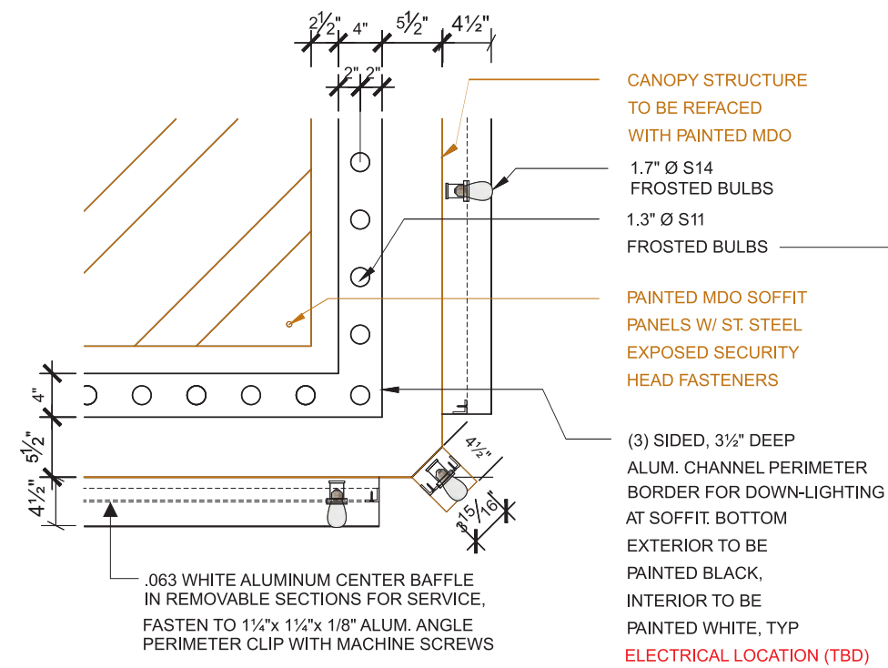
7 REFLECTED CEILING PLAN DETAIL SCALE: 3/4" = 1'-0"
