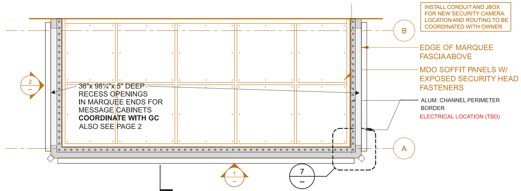
6 REFLECTED CEILING PLAN SCALE: 1/4" = 1'-0"
