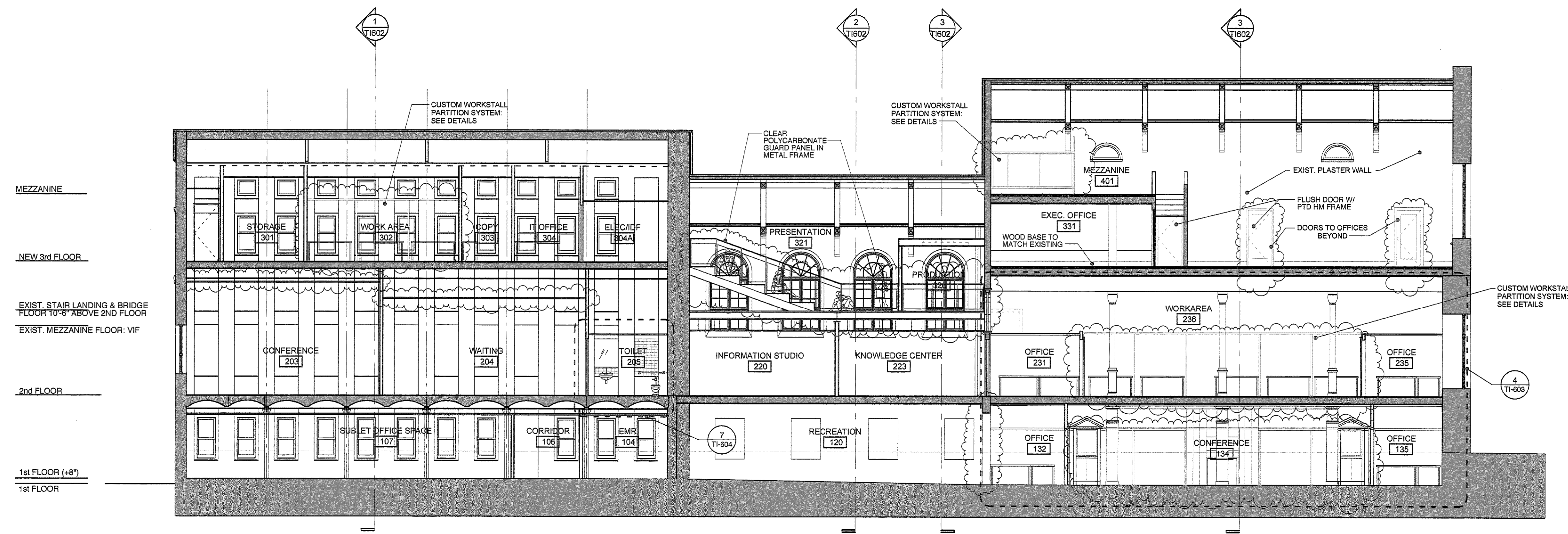
2 BUILDING SECTION THROUGH CENTRAL READING ROOM @ SEATING & PRODUCTION ROOM SCALE: 1/8" = 1'-0"
