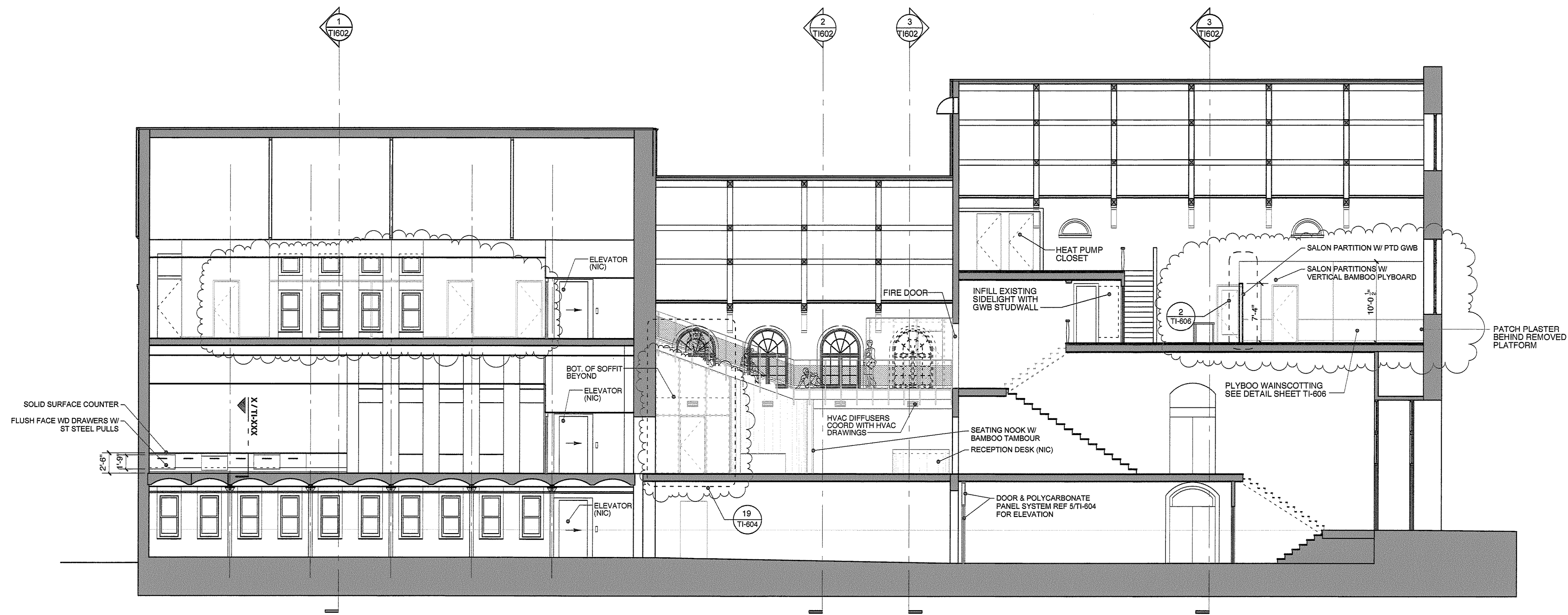
1 BUILDING SECTION THROUGH CENTRAL READING ROOM @ NEW STEPPED CIRCULATION SCALE: 1/8" = 1'-0"
