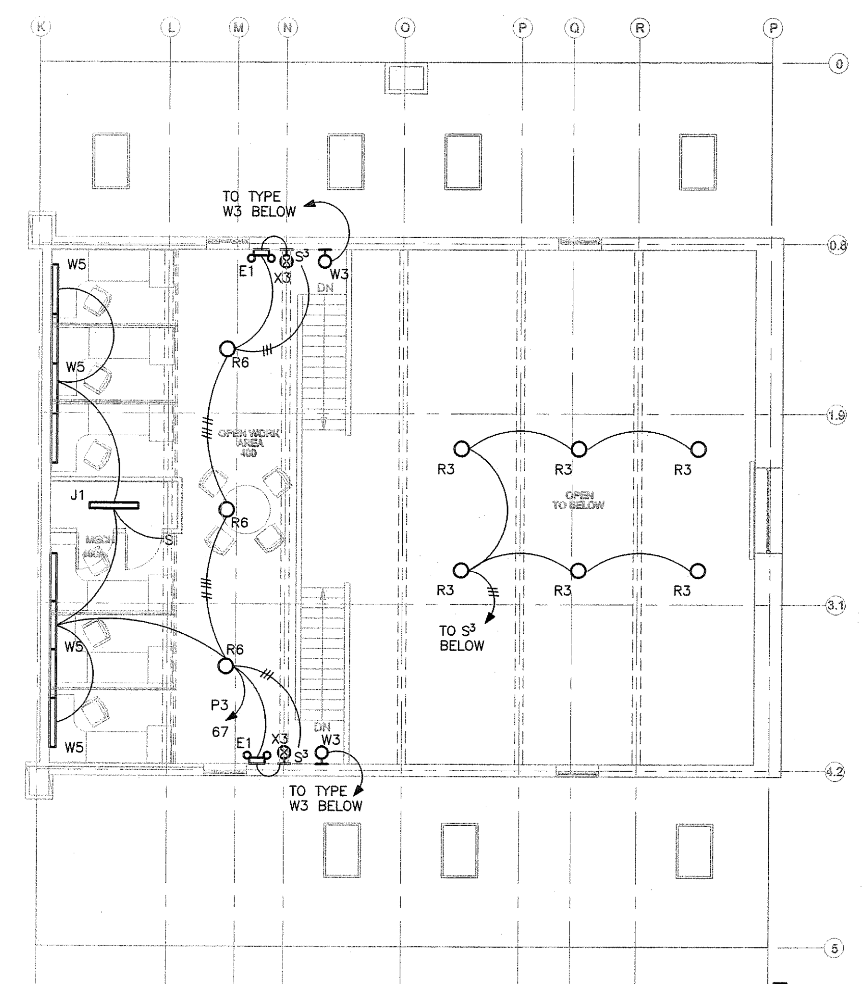
MEZZANINE 1/8" = 1'-0"
