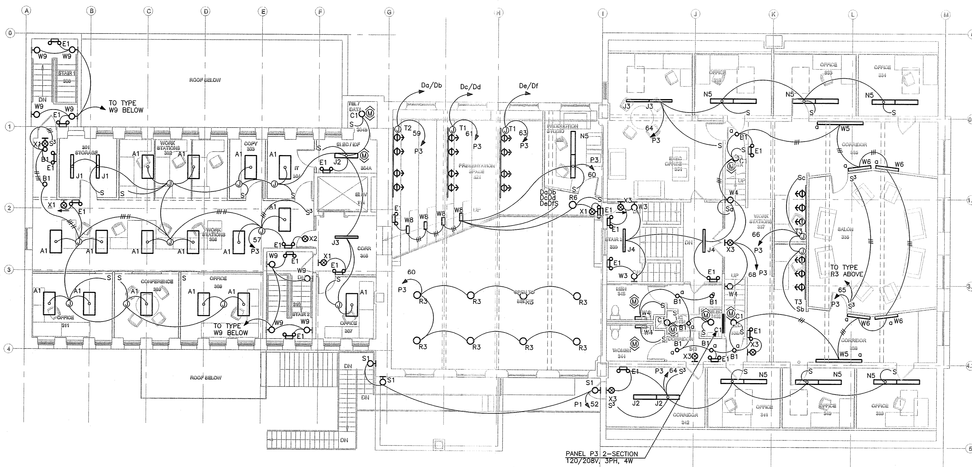
THIRD FLOOR 1/8" = 1'-0"
