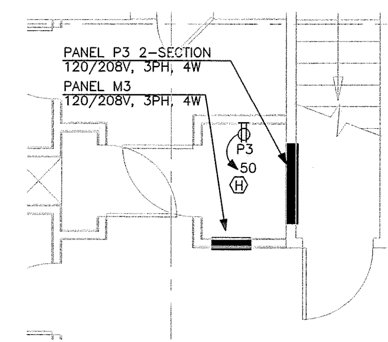
ELEC 343B 1/4" = 1'-0"
