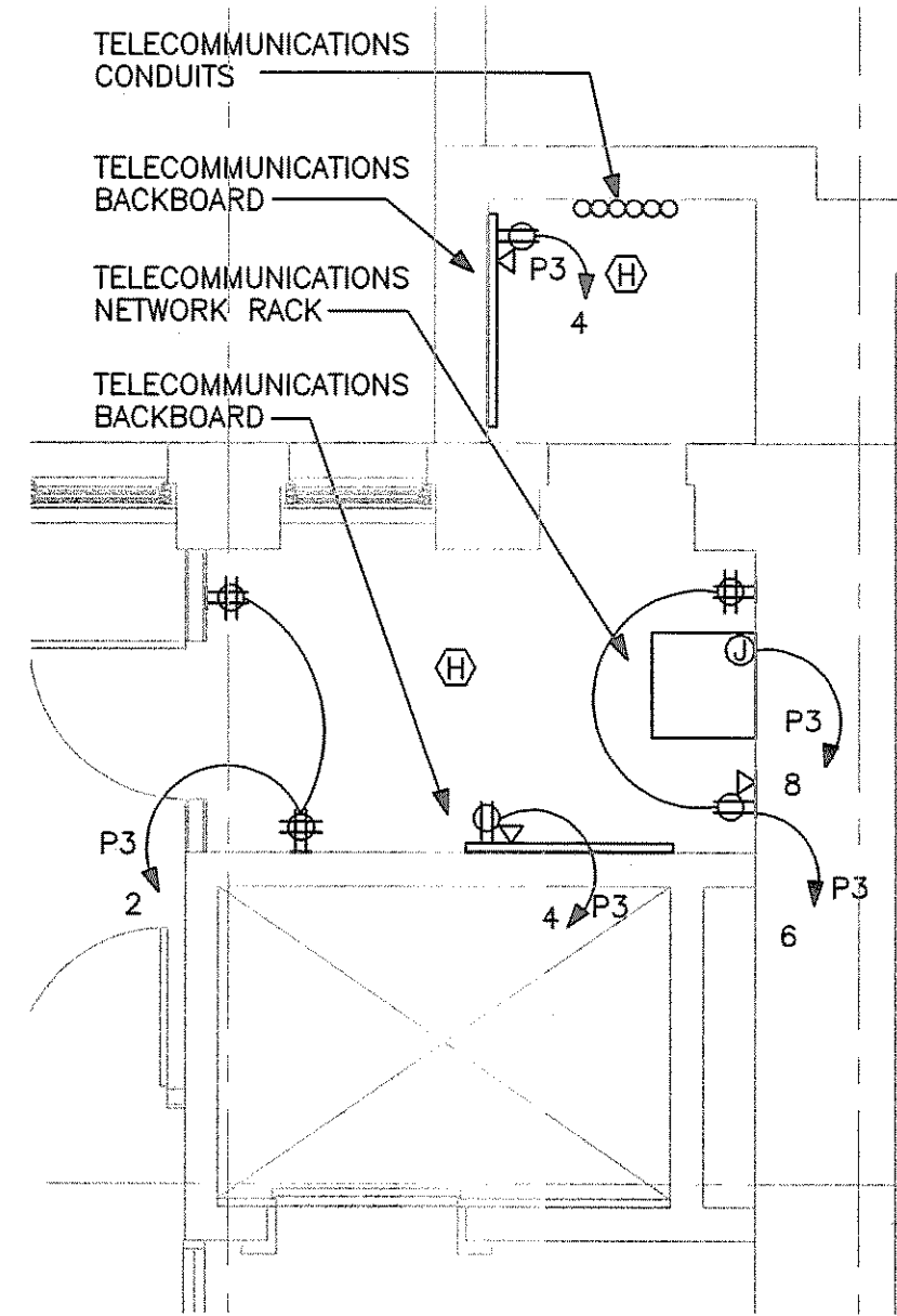
ELEC/IDF 304A & TELE/DATA 304B 1/4" = 1'-0"
