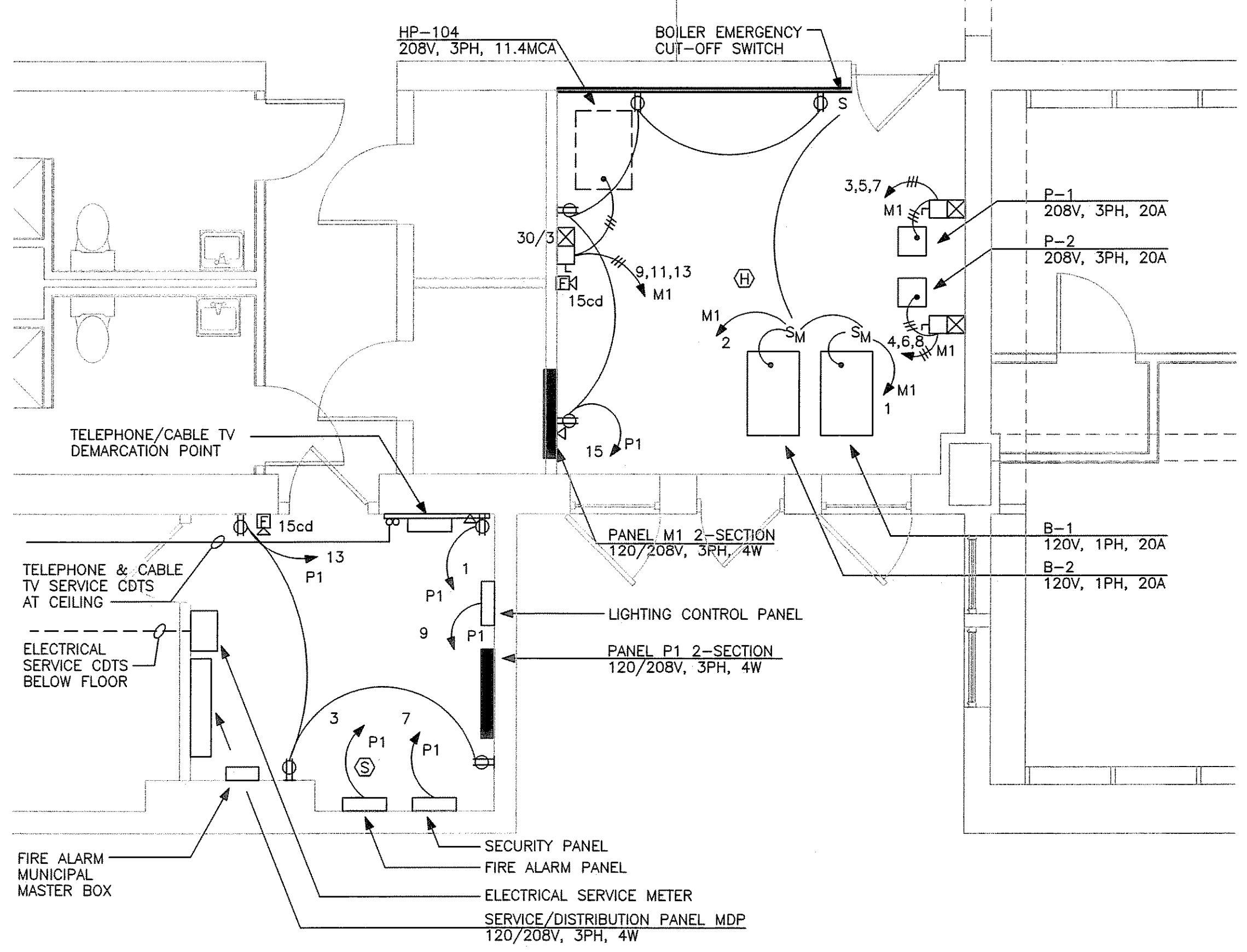
MECHANICAL 122 & ELECTRICAL 126 1/4" = 1'-0"
