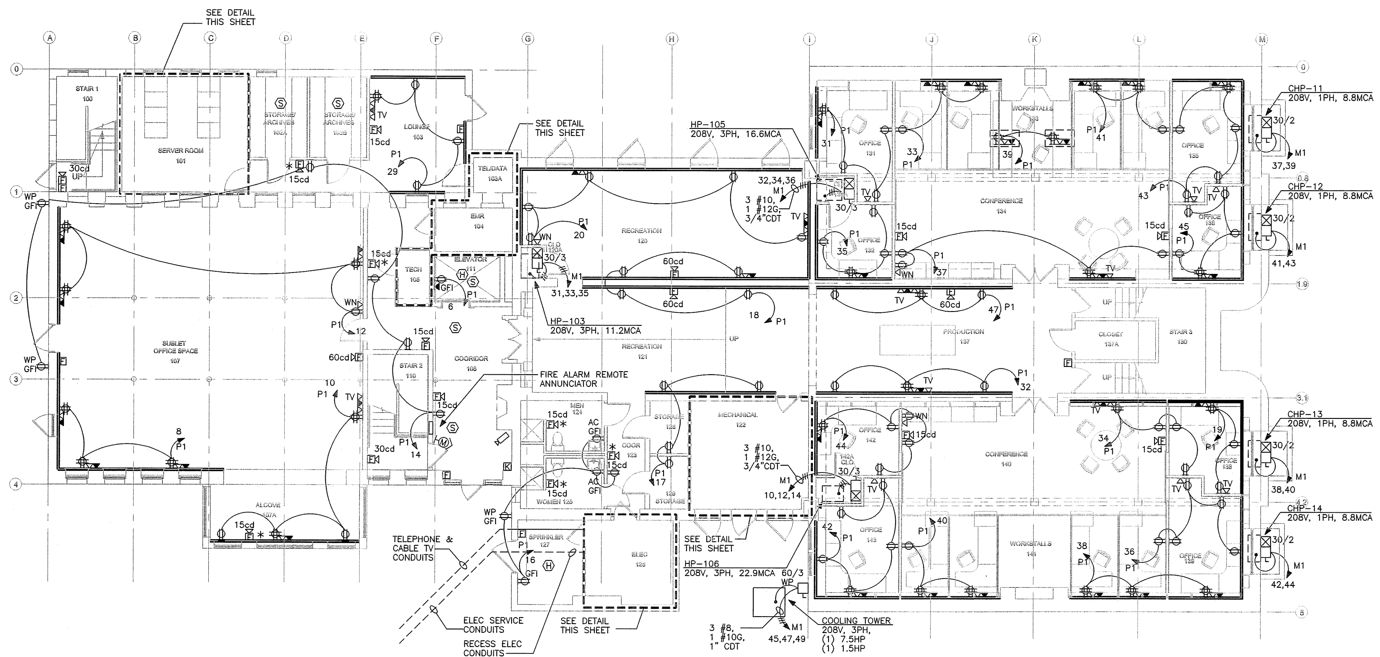
FIRST FLOOR 1/8" = 1'-0"
