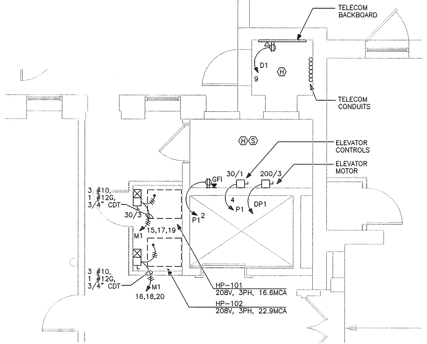
TELE/DATA 103A & EMR 104 & TECH 105 1/4" = 1'-0"
