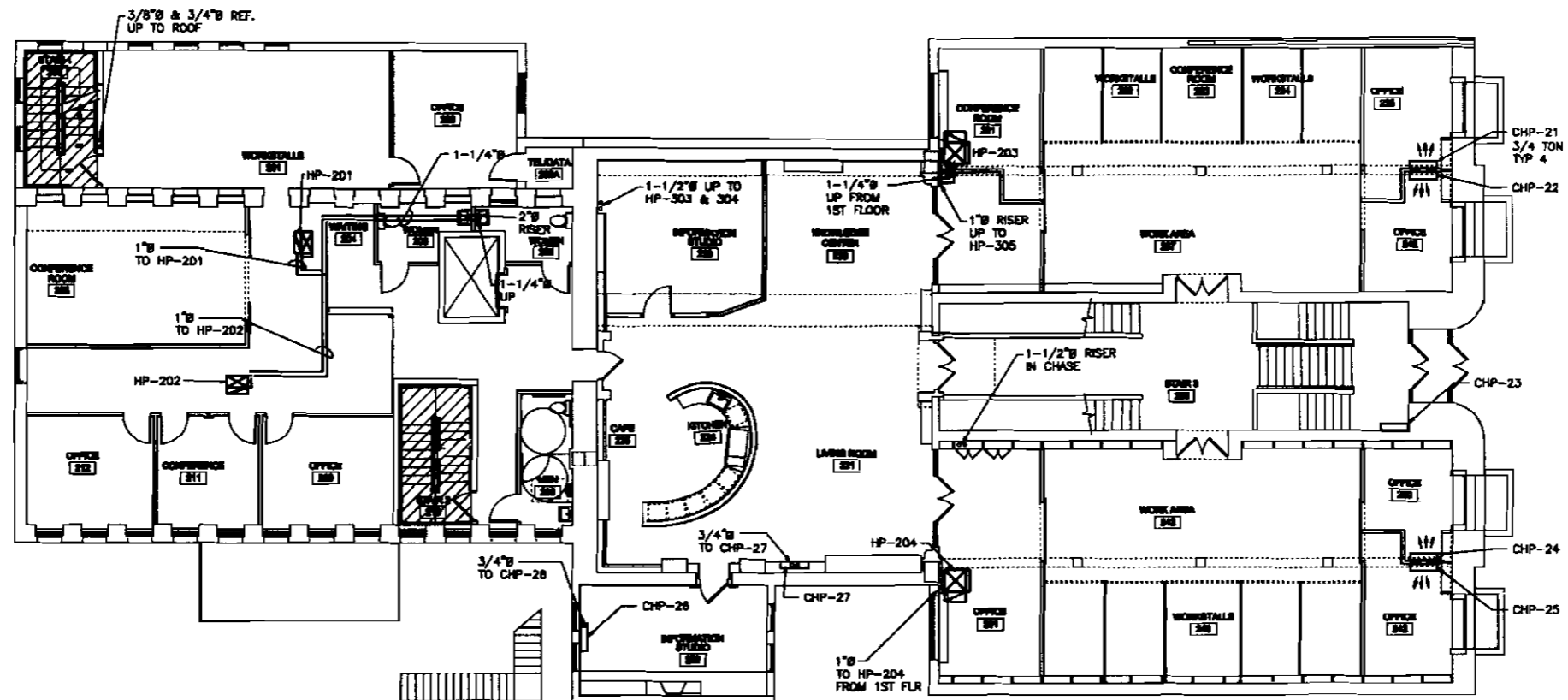
PIPING - SECOND FLOOR PLAN SCALE: 1/8"=1'-0"
