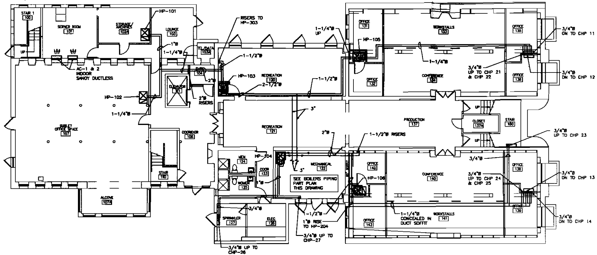
PIPING - FIRST FLOOR PLAN SCALE: 1/8"=1'-0"
