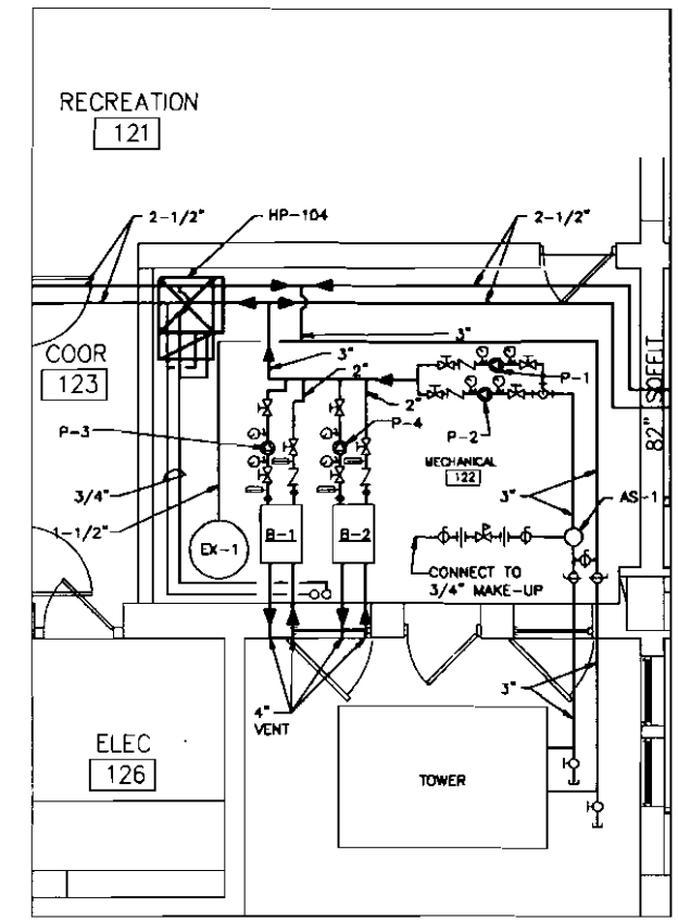
BOILERS PIPING PLAN SCALE: 1/4"=1'-0"
