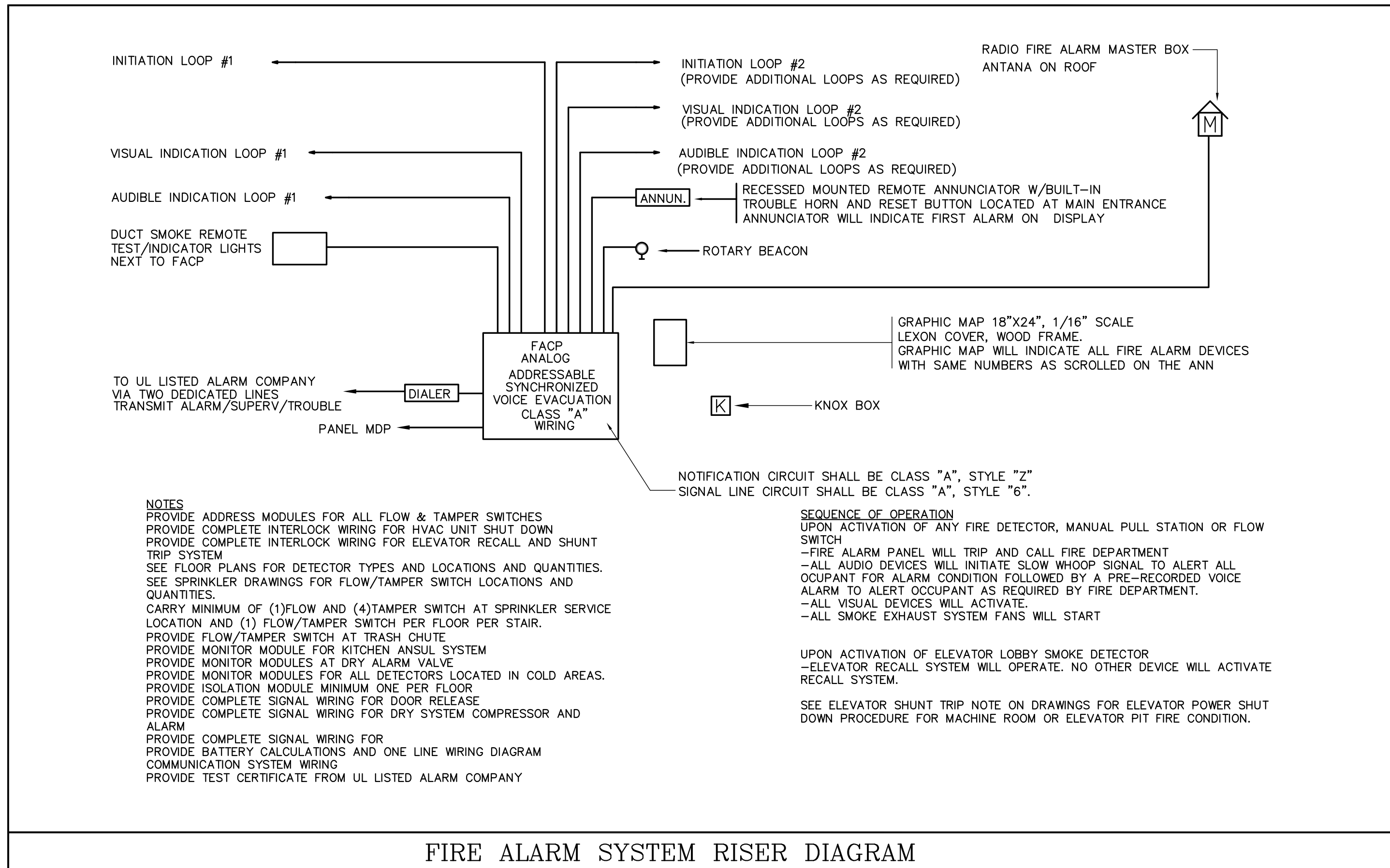
FIRE ALARM SYSTEM RISER DIAGRAM
