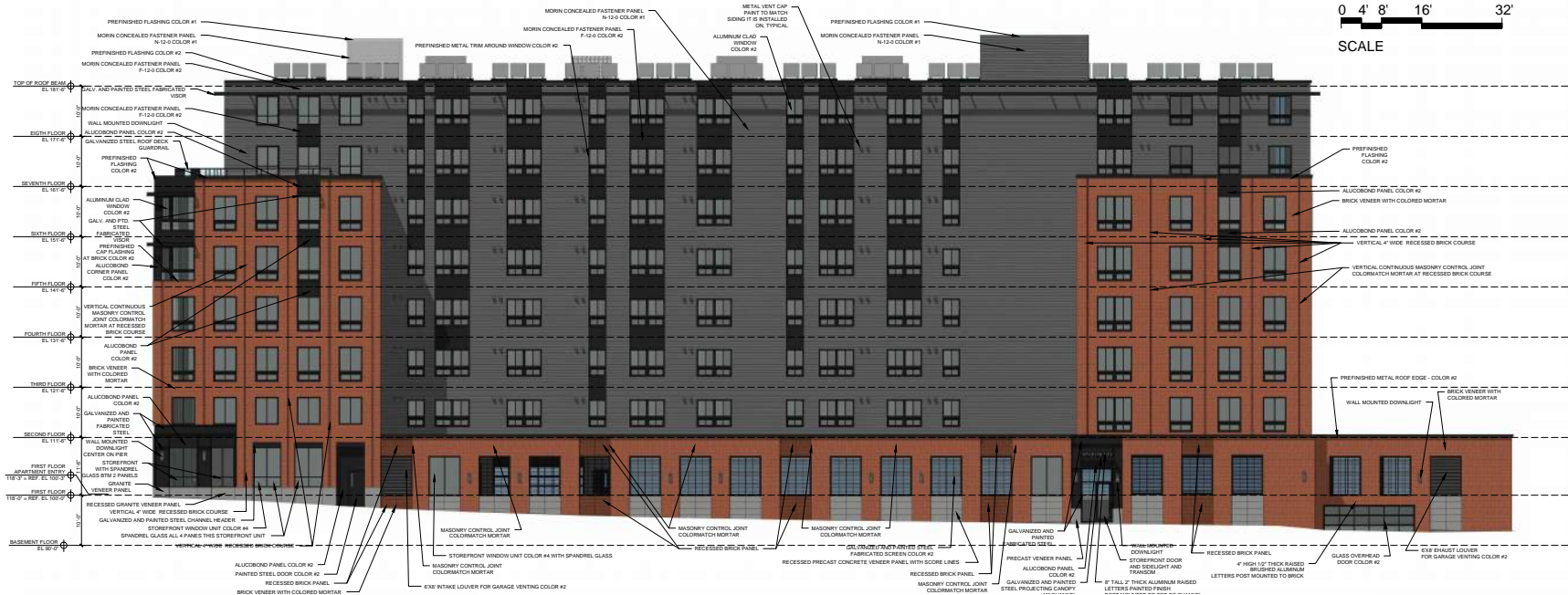
2 EAST ELEVATION
