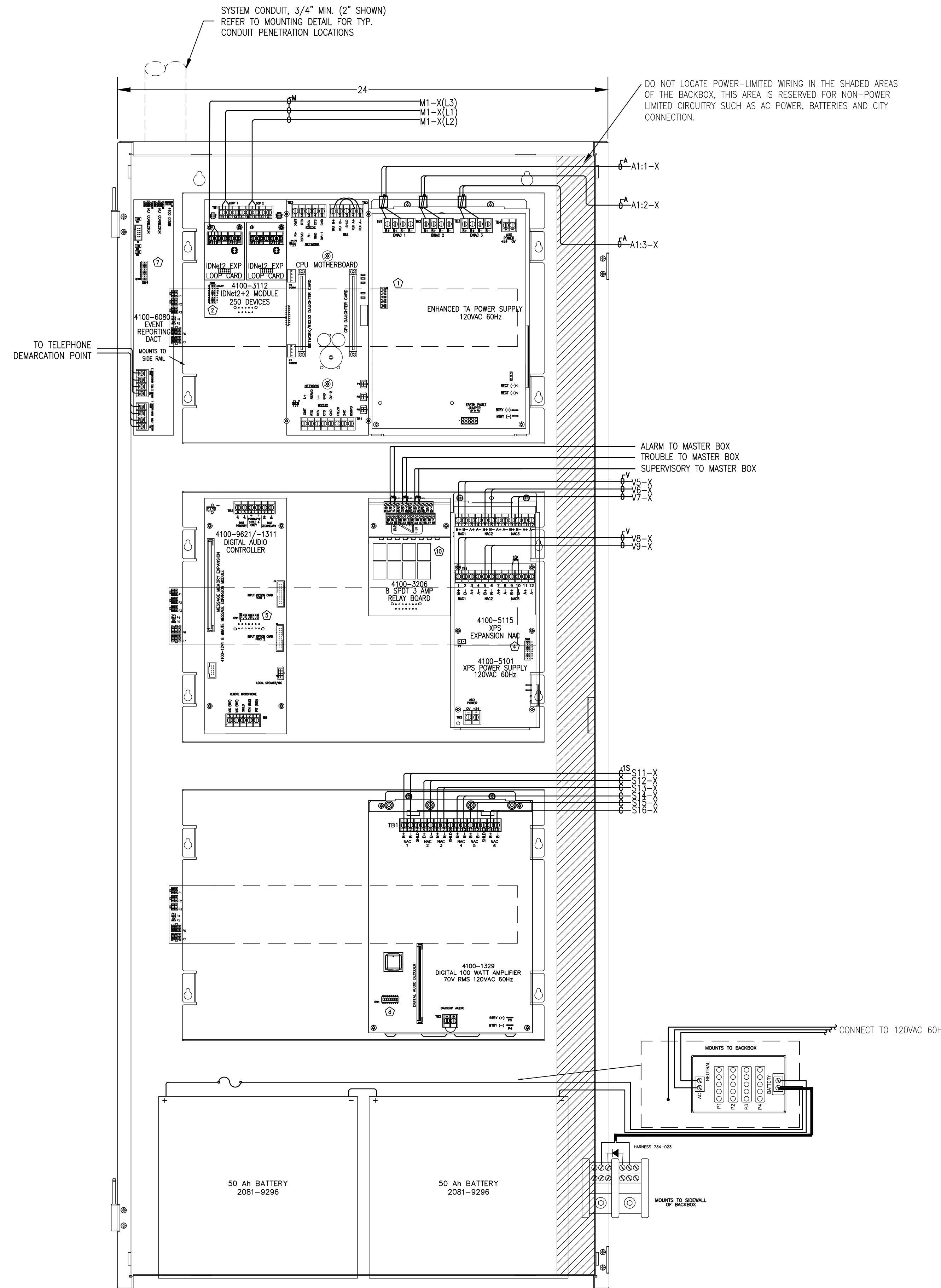
PANEL DETAIL - 4100ES PANEL SCALE: NTS
