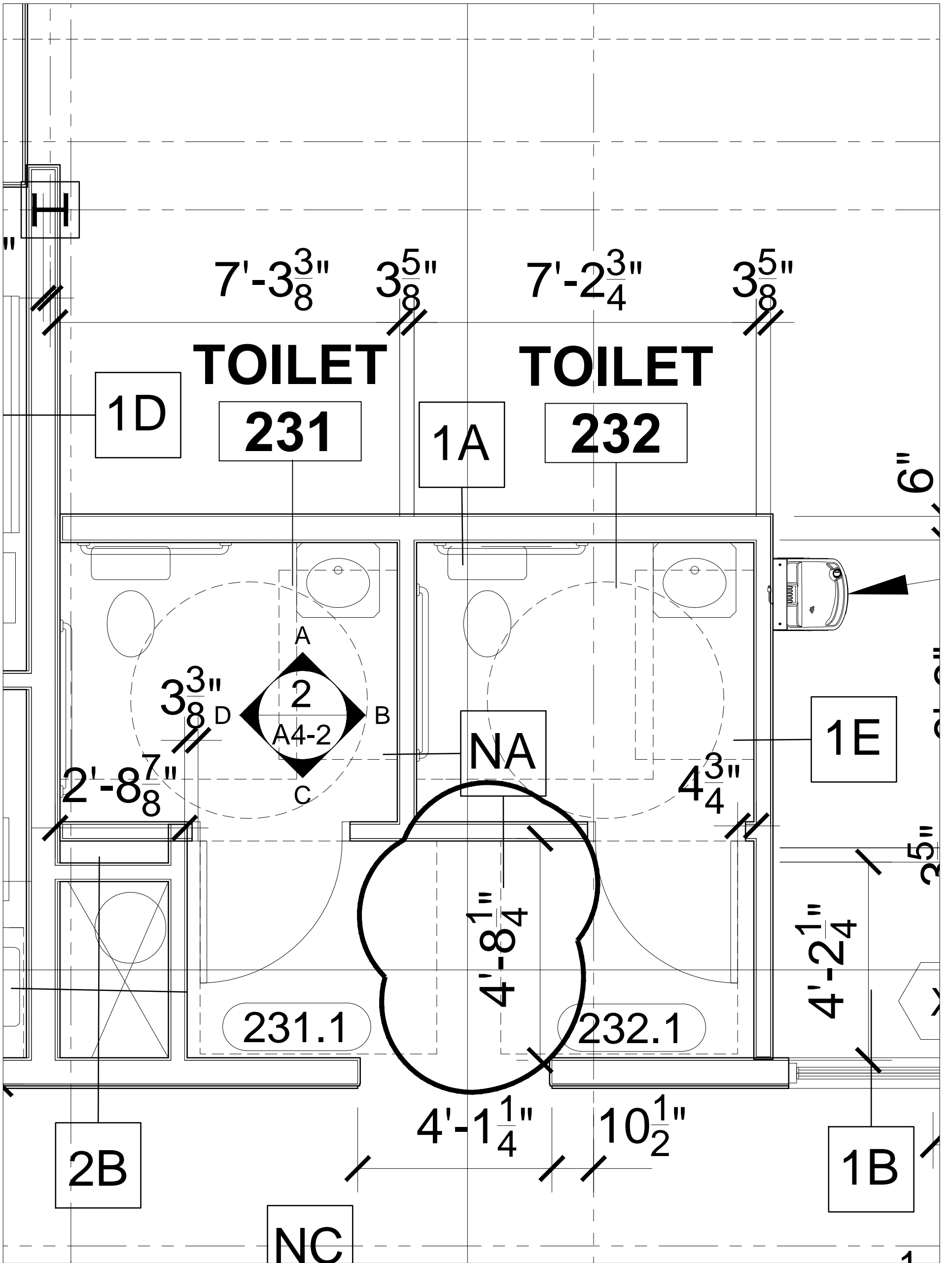
1 TOILET ROOM PLAN 1/2" = 1'-0"
