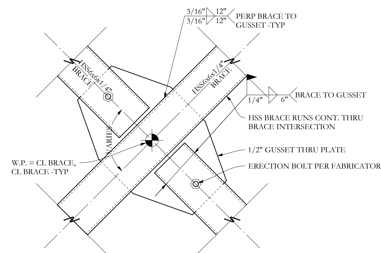
SECTION D 1 1/2"=1'-0" TYPICAL HSS6x6x1/4 BRACE MID CONN
