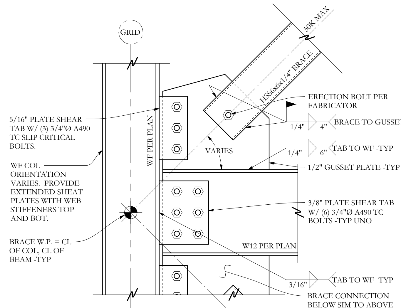
SECTION A 1 1/2"=1'-0" TYPICAL HSS6x6x1/4 BRACE END CONN
