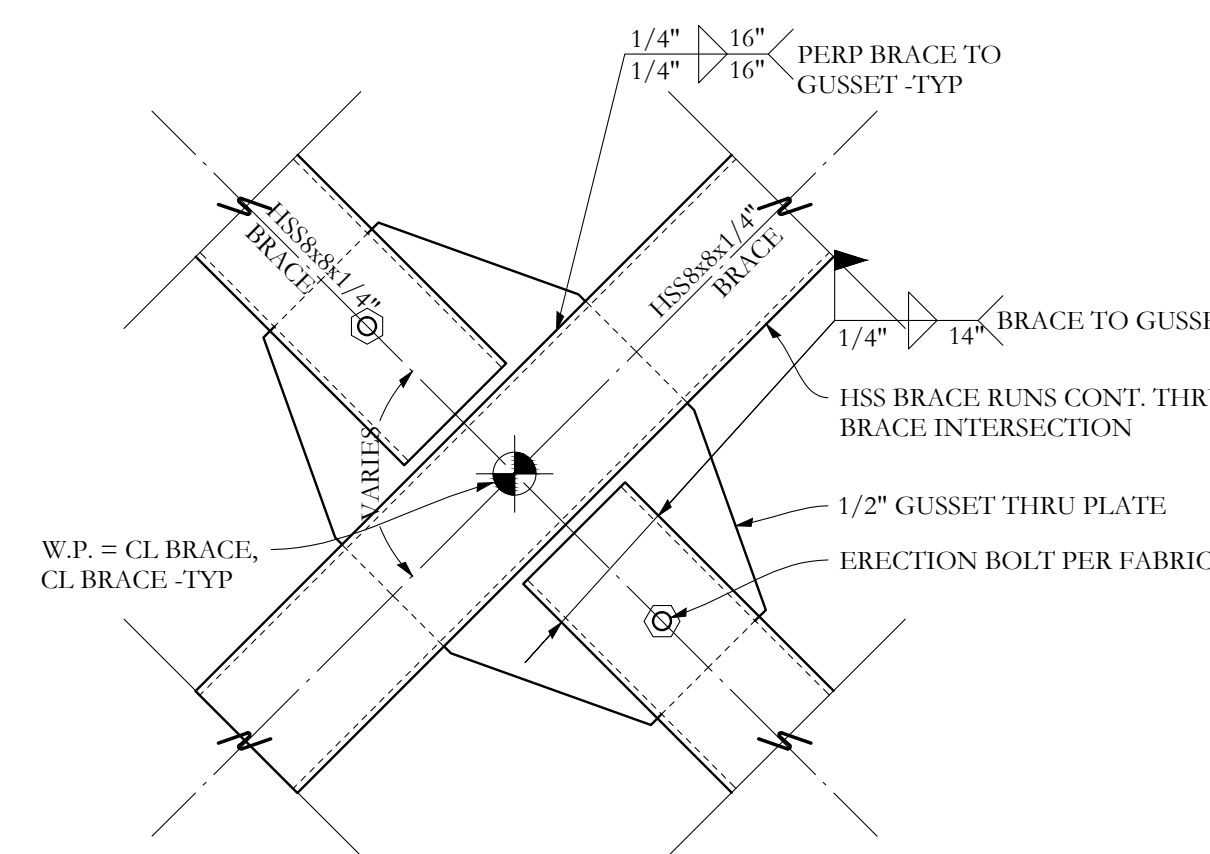
SECTION F 1 1/2"=1'-0" TYPICAL HSS8x8x1/4 BRACE MID CONN
