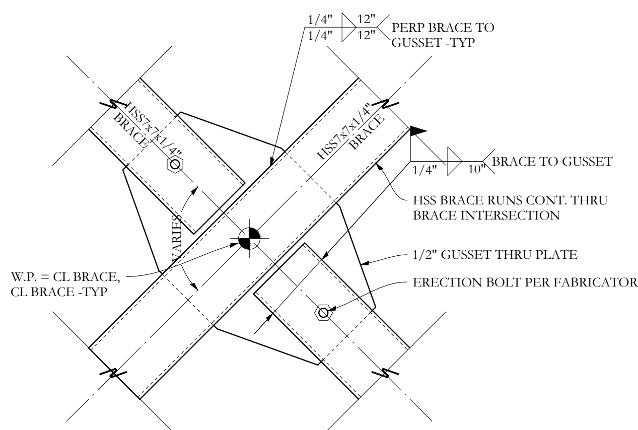
SECTION E 1 1/2"=1'-0" TYPICAL HSS7x7x1/4 BRACE MID CONN
