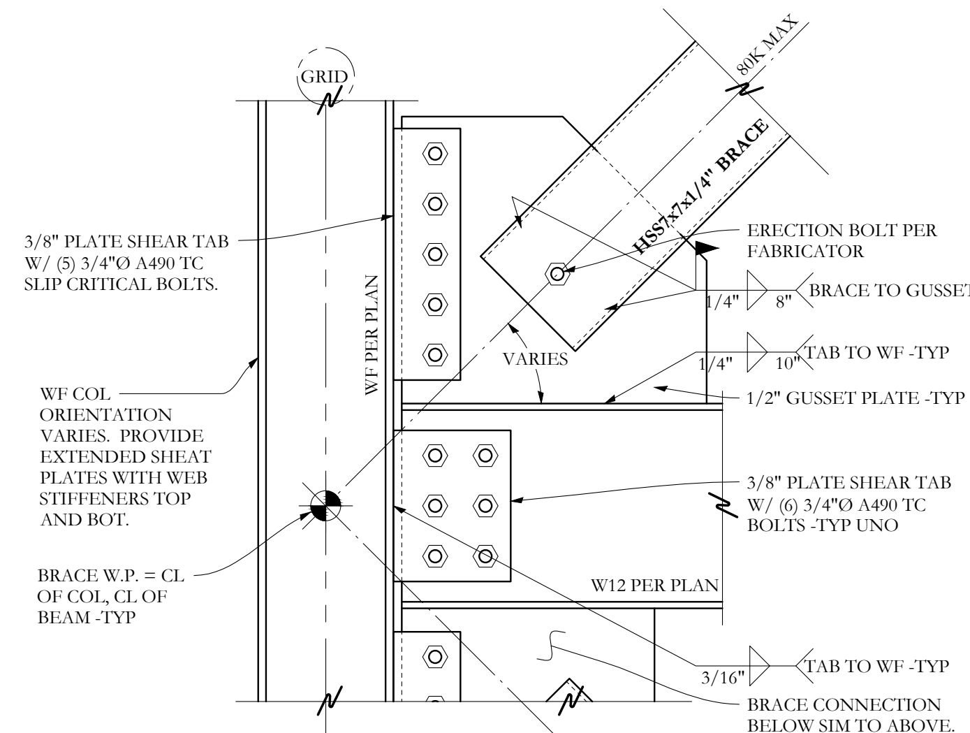
SECTION B 1 1/2"=1'-0" TYPICAL HSS7x7x1/4 BRACE END CONN
