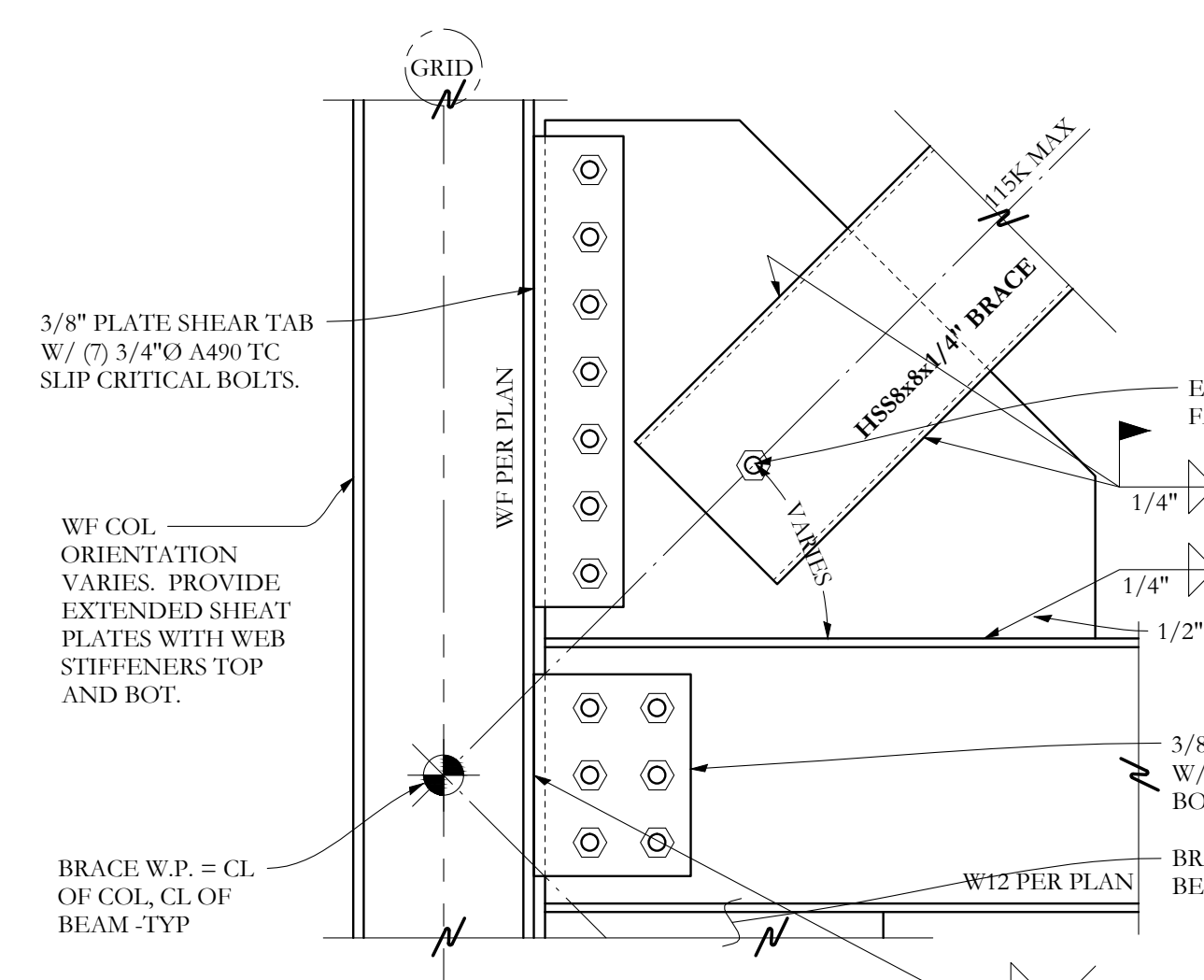
SECTION C 1 1/2"=1'-0" TYPICAL HSS8x8x1/4 BRACE END CONN
