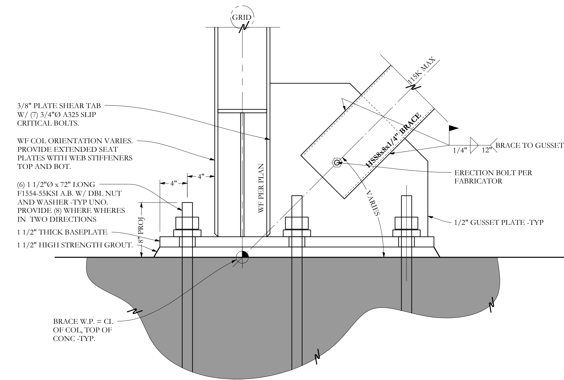
SECTION G 1 1/2"=1'-0" TYPICAL BRACE CONN TO MASS FTG
