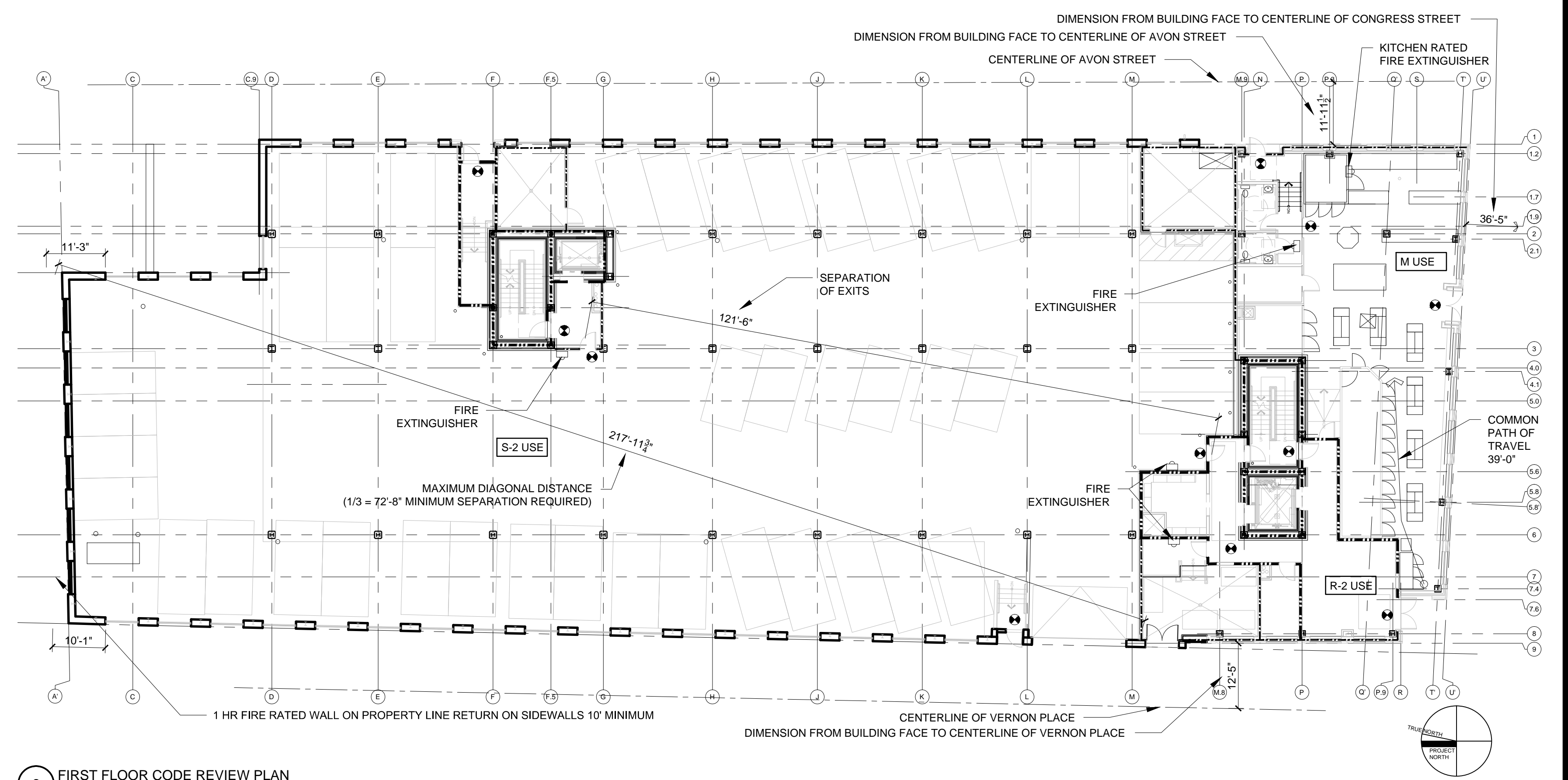
2 FIRST FLOOR CODE REVIEW PLAN 1/16" = 1'-0"
