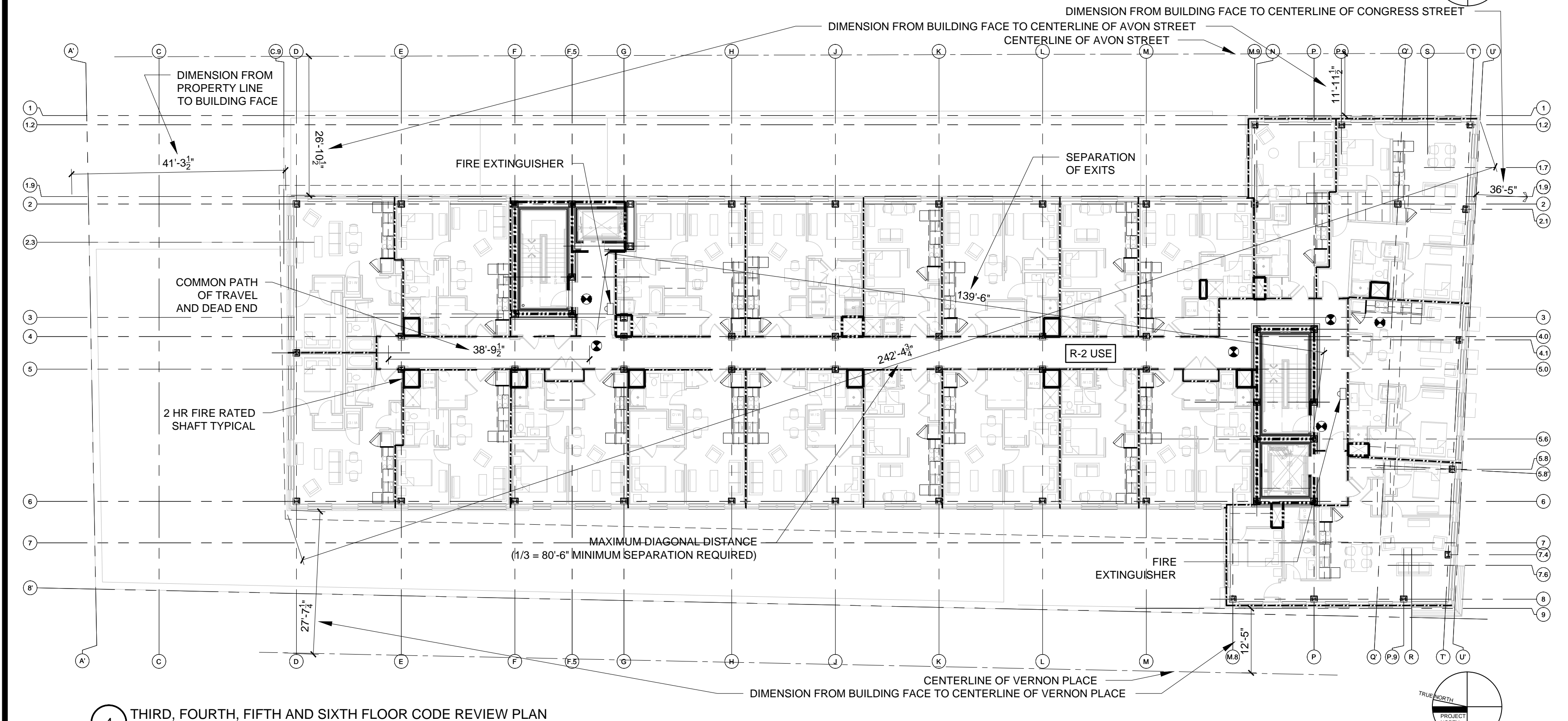
4 THIRD, FOURTH, FIFTH AND SIXTH FLOOR CODE REVIEW PLAN 1/16" = 1'-0"
