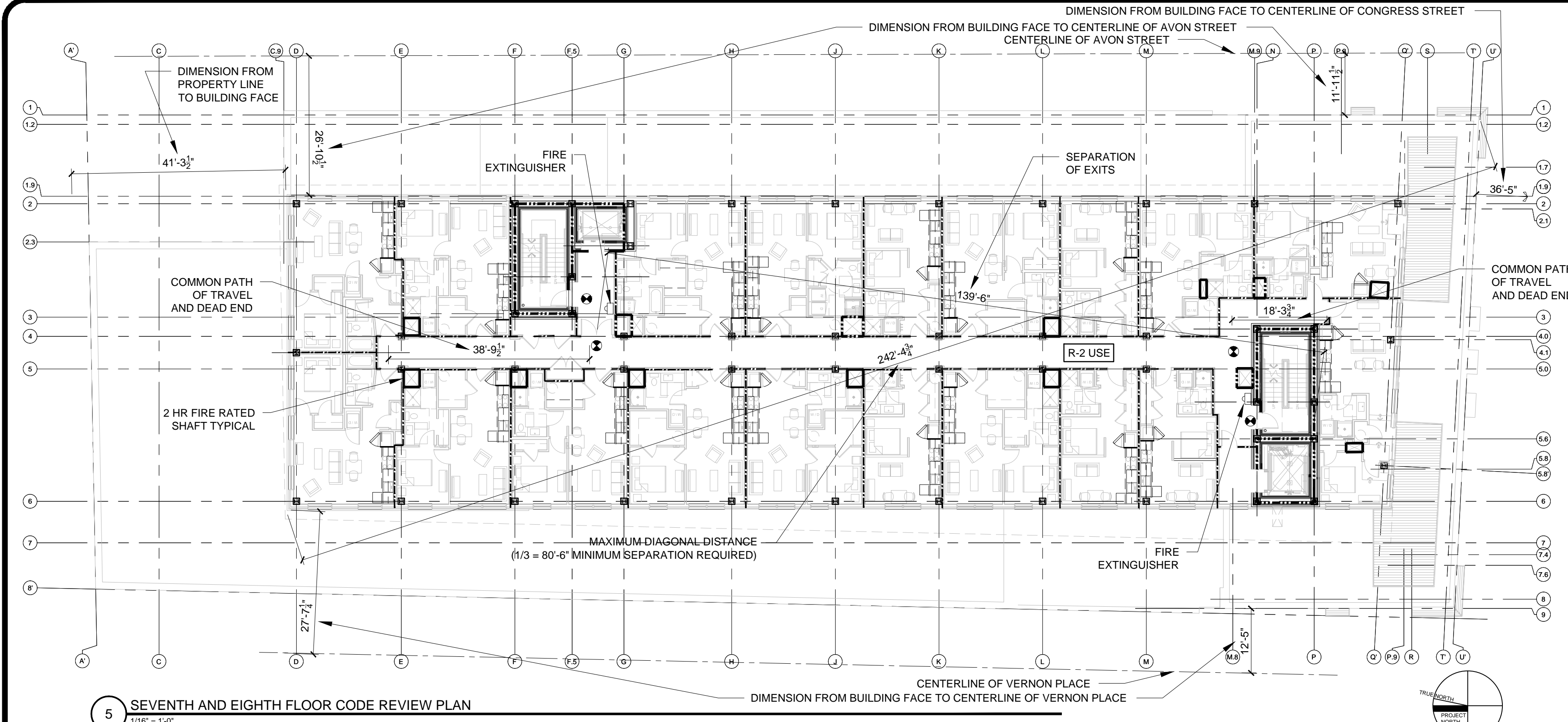
5 SEVENTH AND EIGHTH FLOOR CODE REVIEW PLAN 1/16" = 1'-0"
