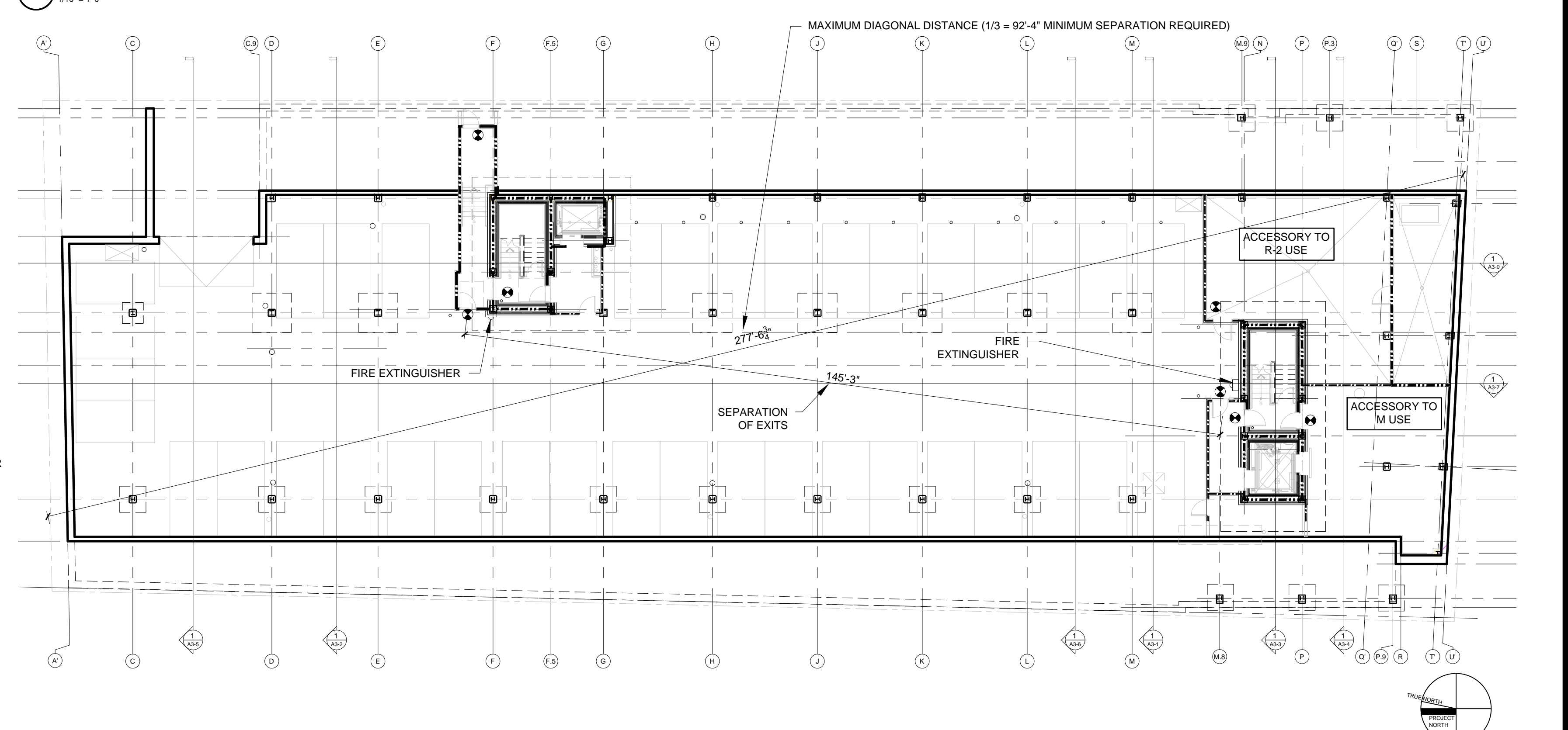
1 BASEMENT CODE REVIEW PLAN 1/16" = 1'-0"
