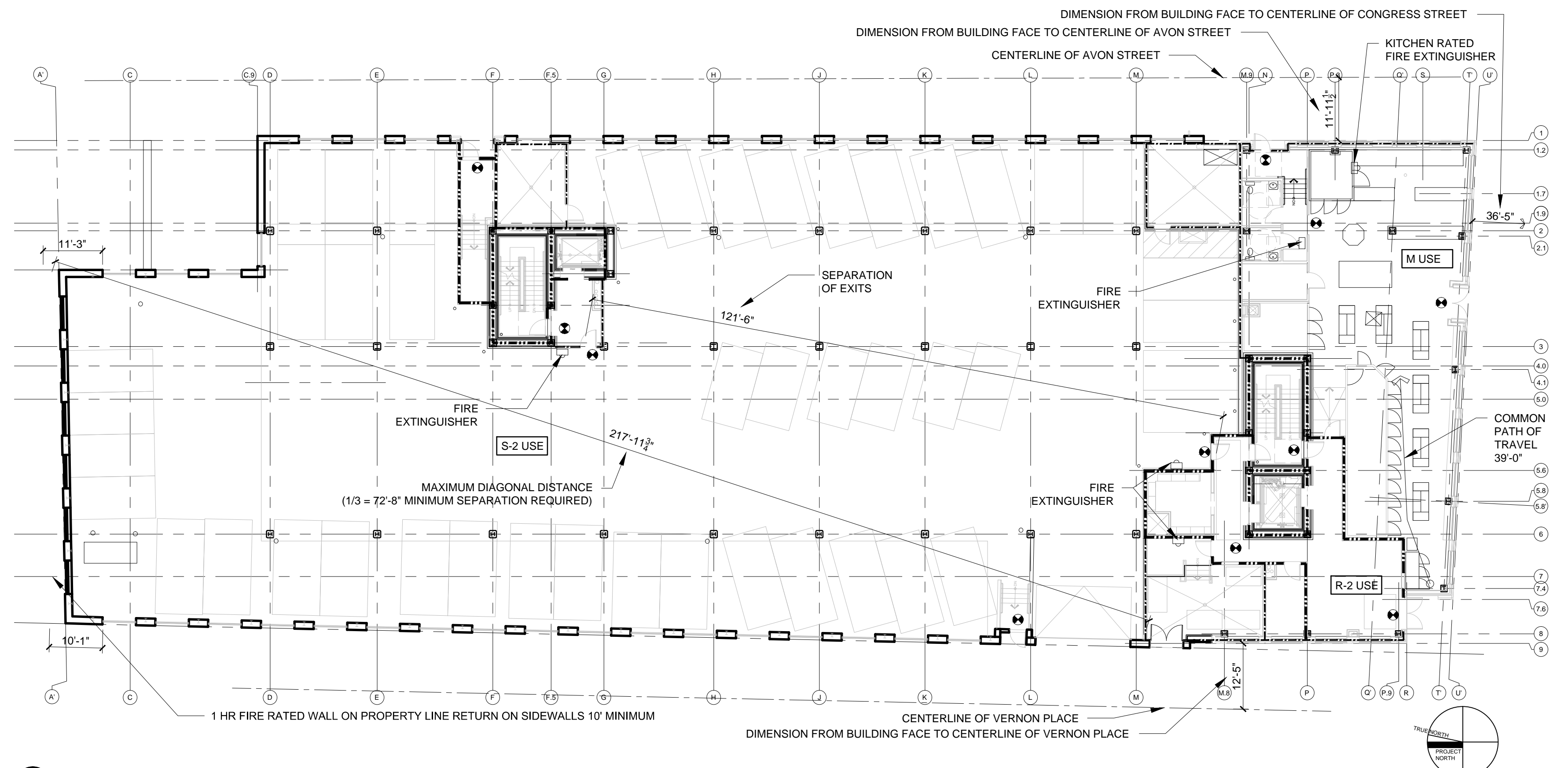
2 FIRST FLOOR CODE REVIEW PLAN 1/16" = 1'-0"
