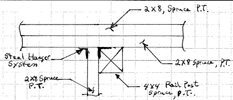
Detail A - Plan B-B
