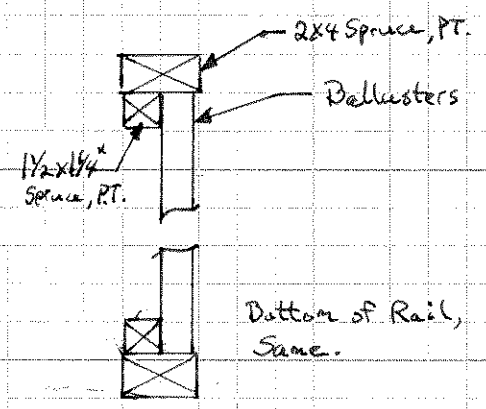
Detail B - Elev.
