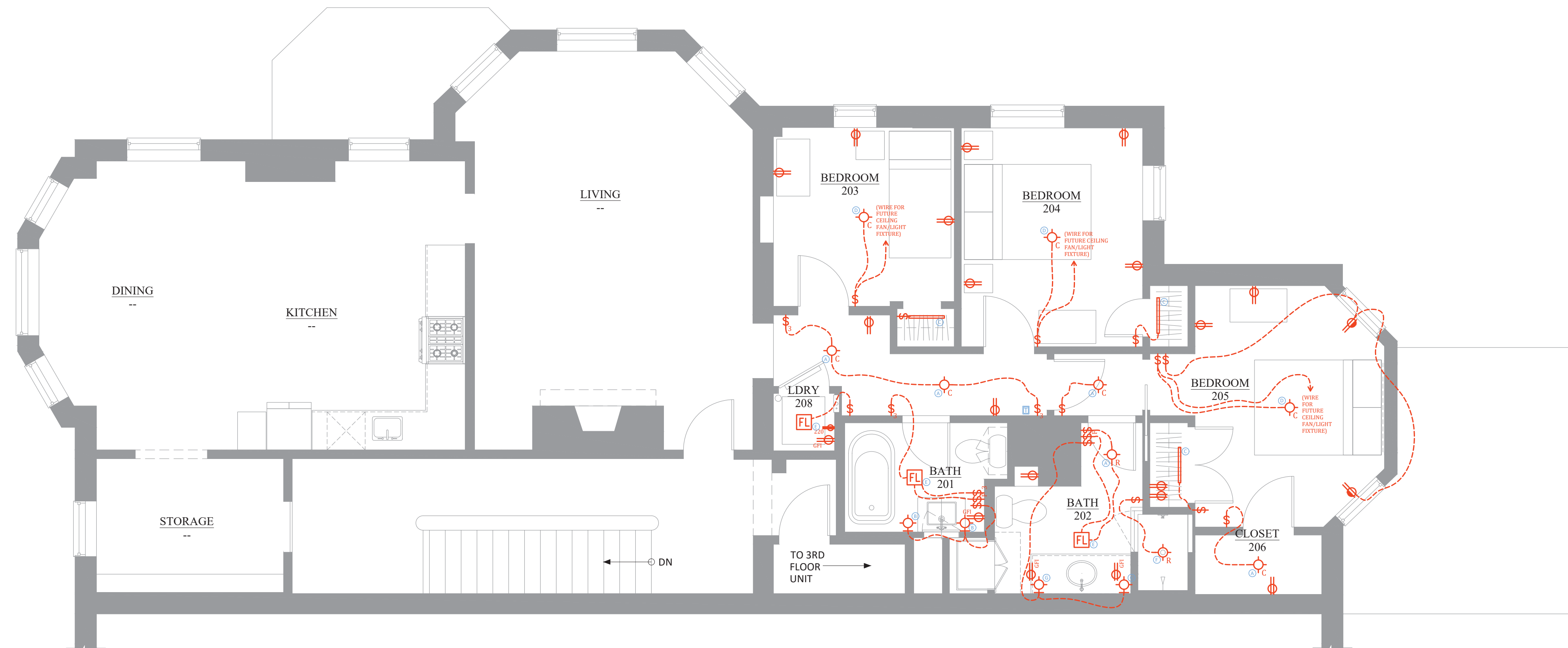
1 ELECTRICAL PLAN 3/4" = 1'-0"
