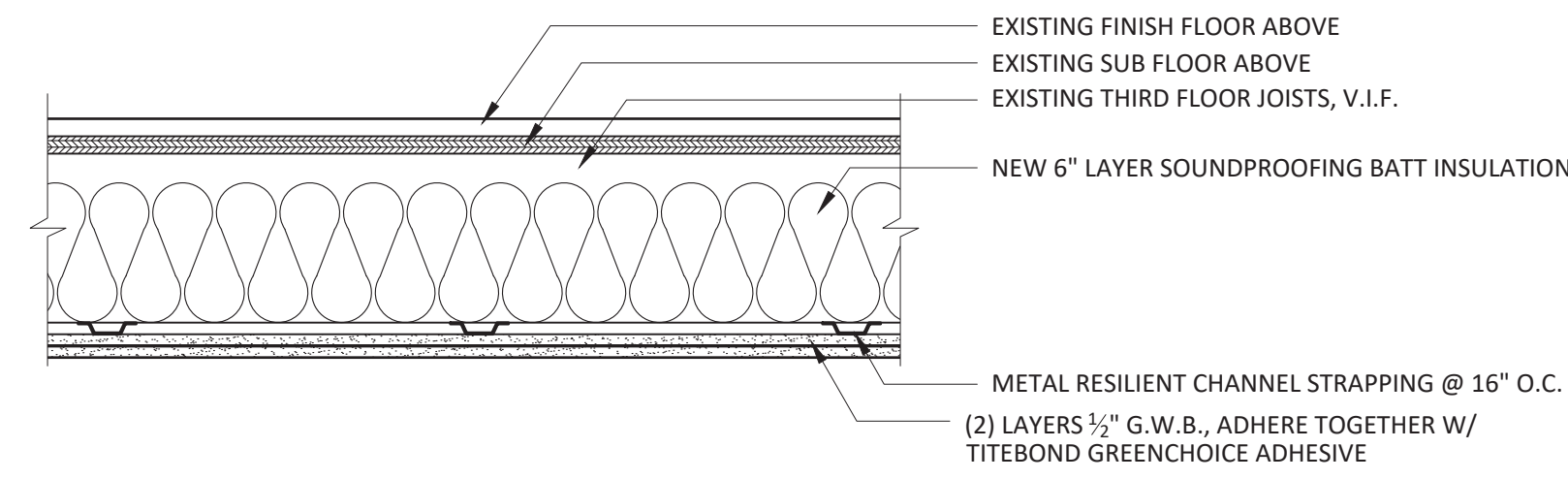
2 CEILING SOUNDPROOFING DETAIL 1 1/2" = 1'-0"
