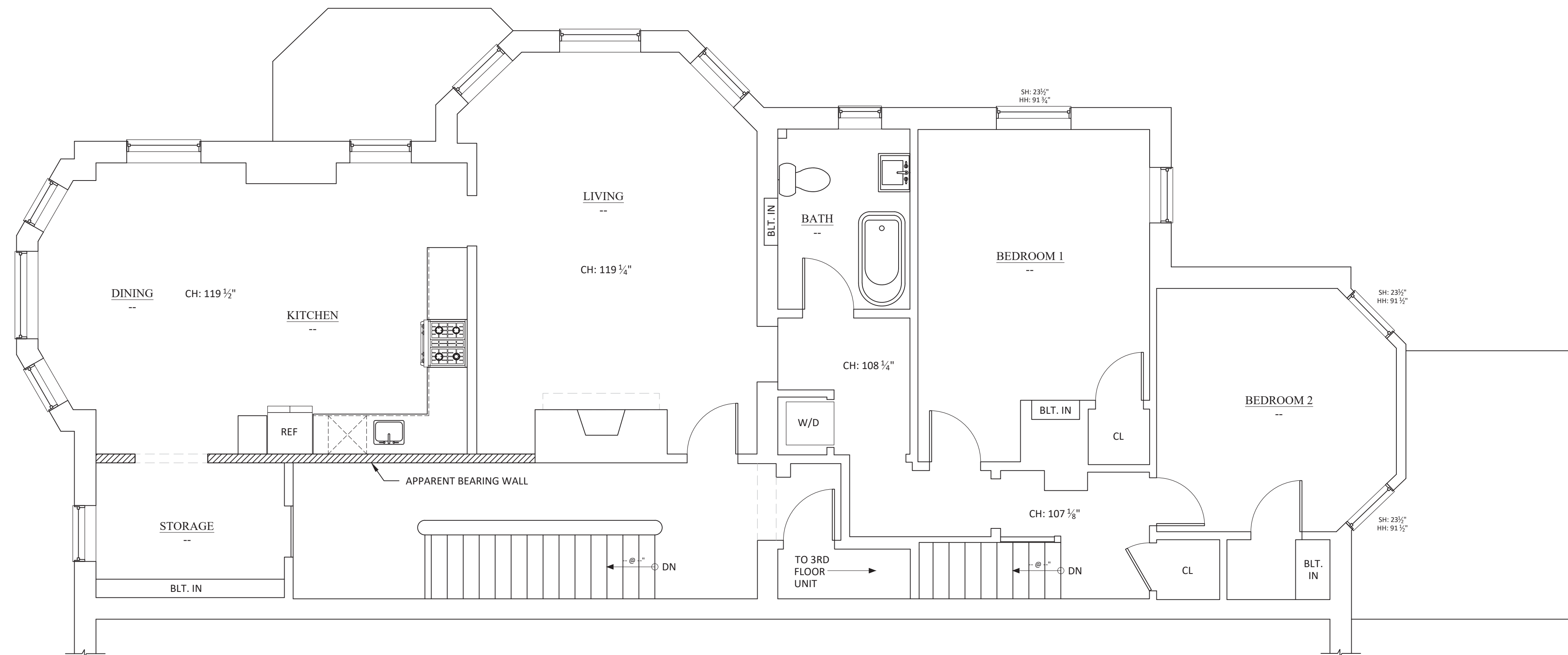
1 EXISTING FLOOR PLAN 1/4" = 1'-0"
