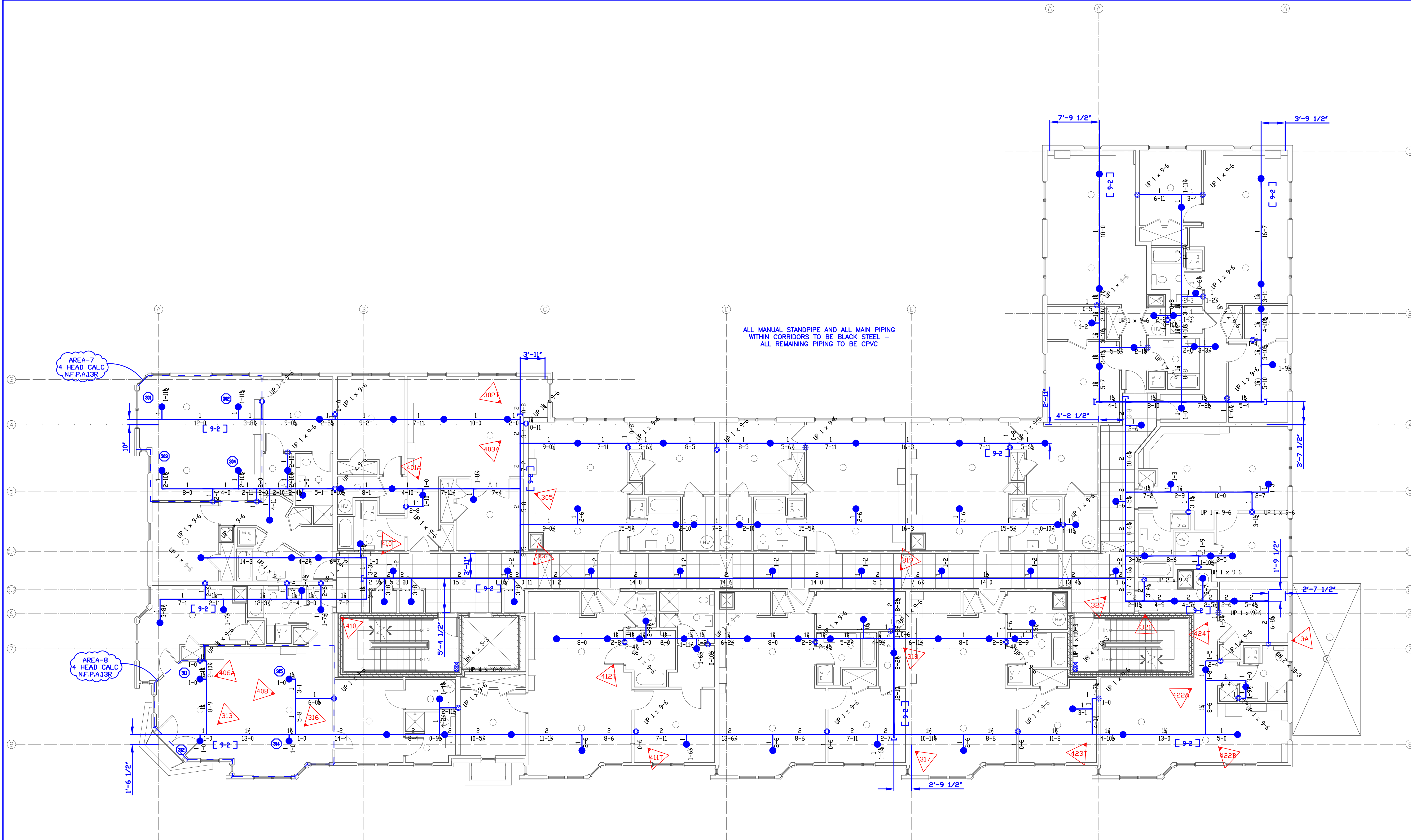
THIRD LEVEL PLAN FINISHED FLOOR ELEV = 165'-3" SCALE: 1/8"=1'-0"
