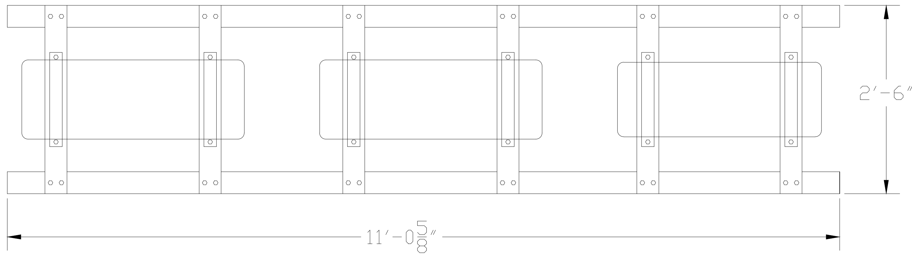
Condenser Mounting Detail
