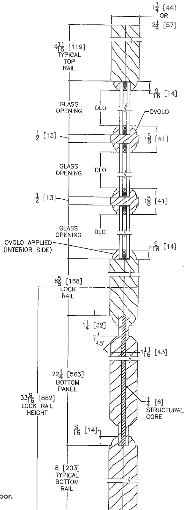
VERTICAL DOOR CROSS SECTION Insulated Glass
