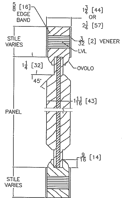
HORIZONTAL DOOR CROSS SECTION Engineered Stile Option (Upon Request or Doors > 8'-0")
