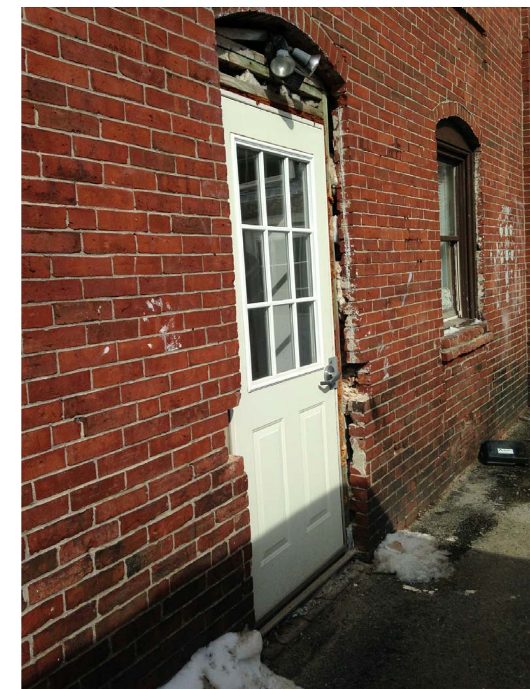
DOOR IN SOUTH FACADE OF 2-STORY BRICK BUILDING
