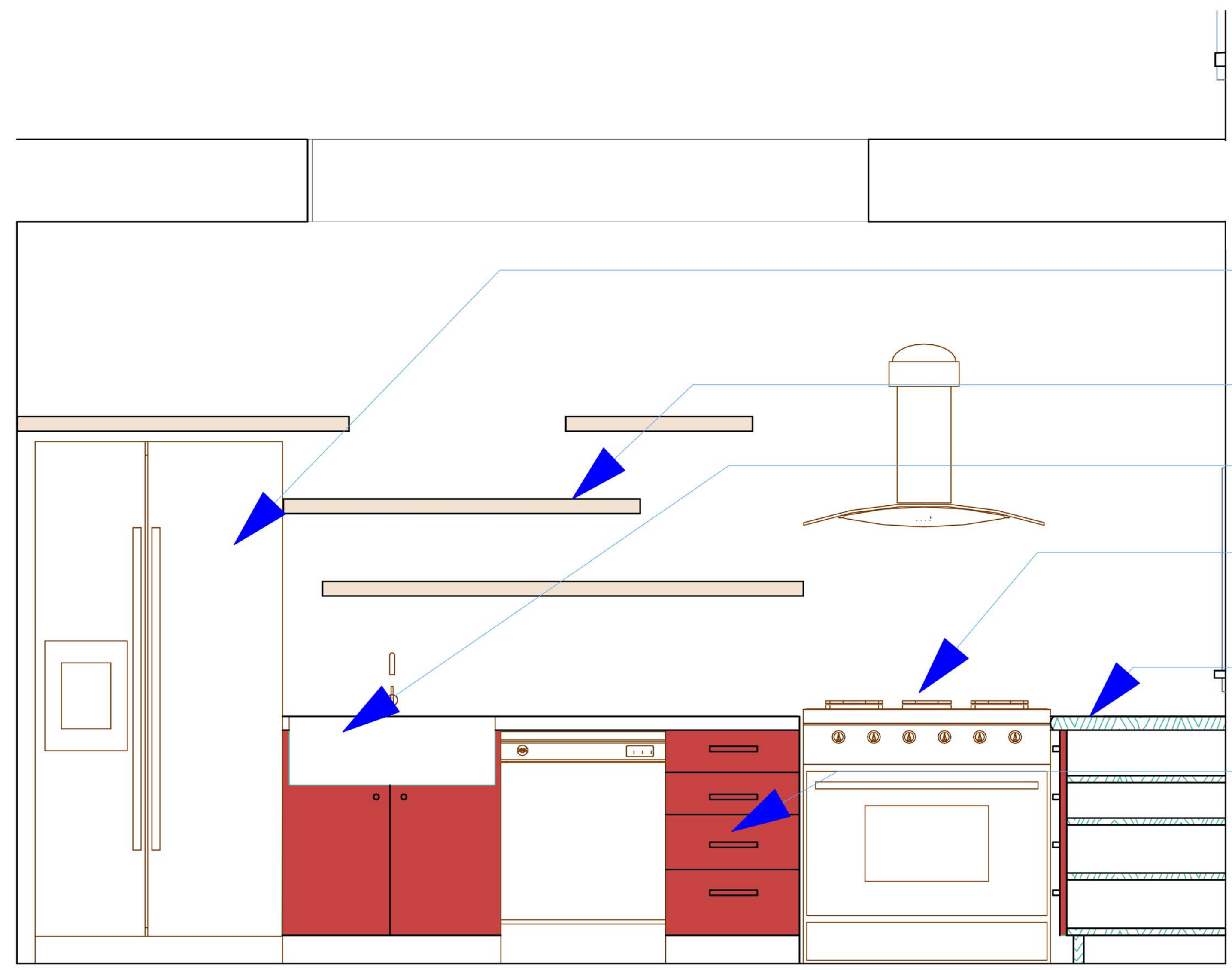
KITCHEN ELEVATION SCALE: 1" = 1'-0"
