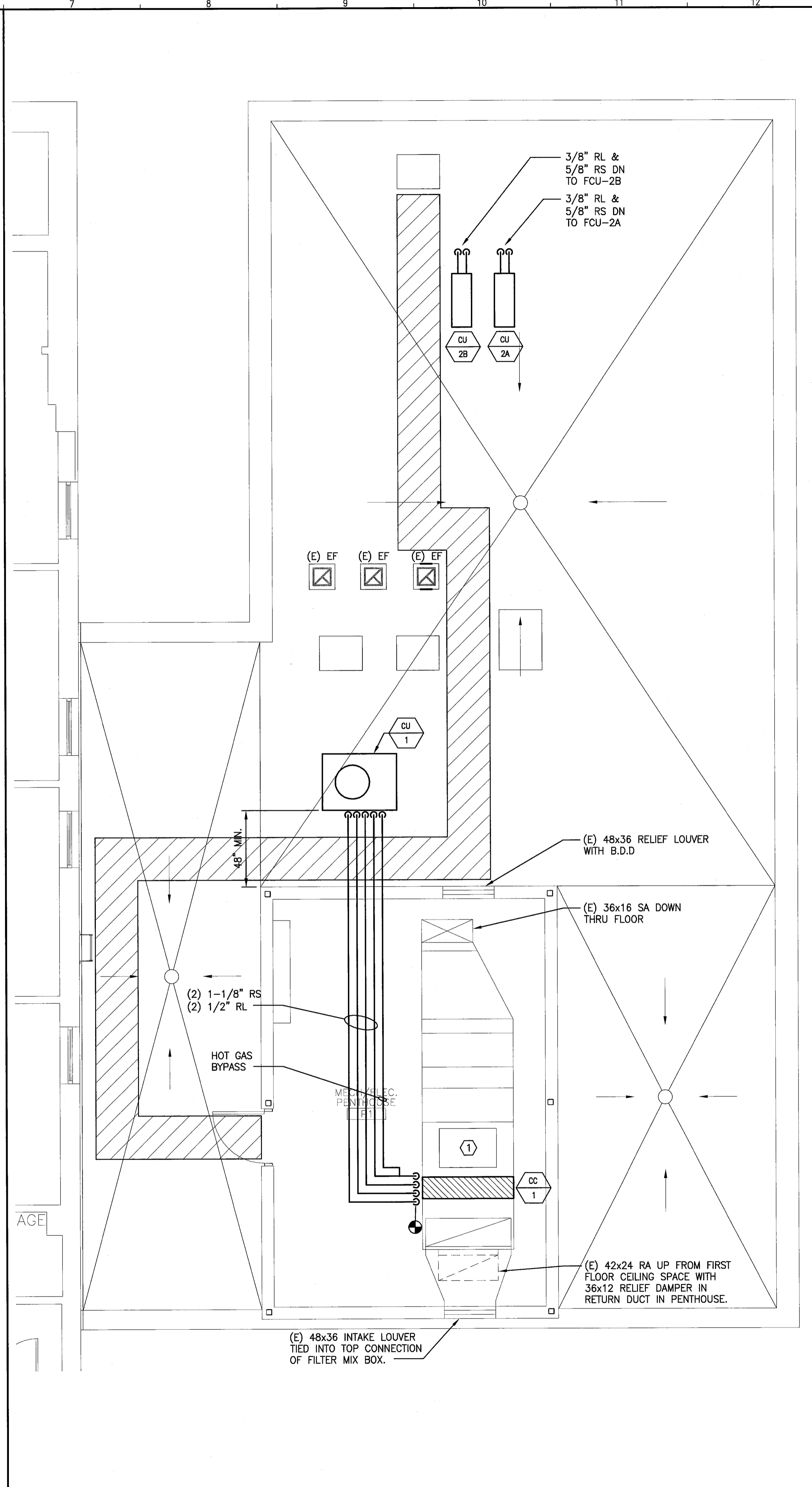
A7 ROOF PLAN 1/4"=1'-0"
