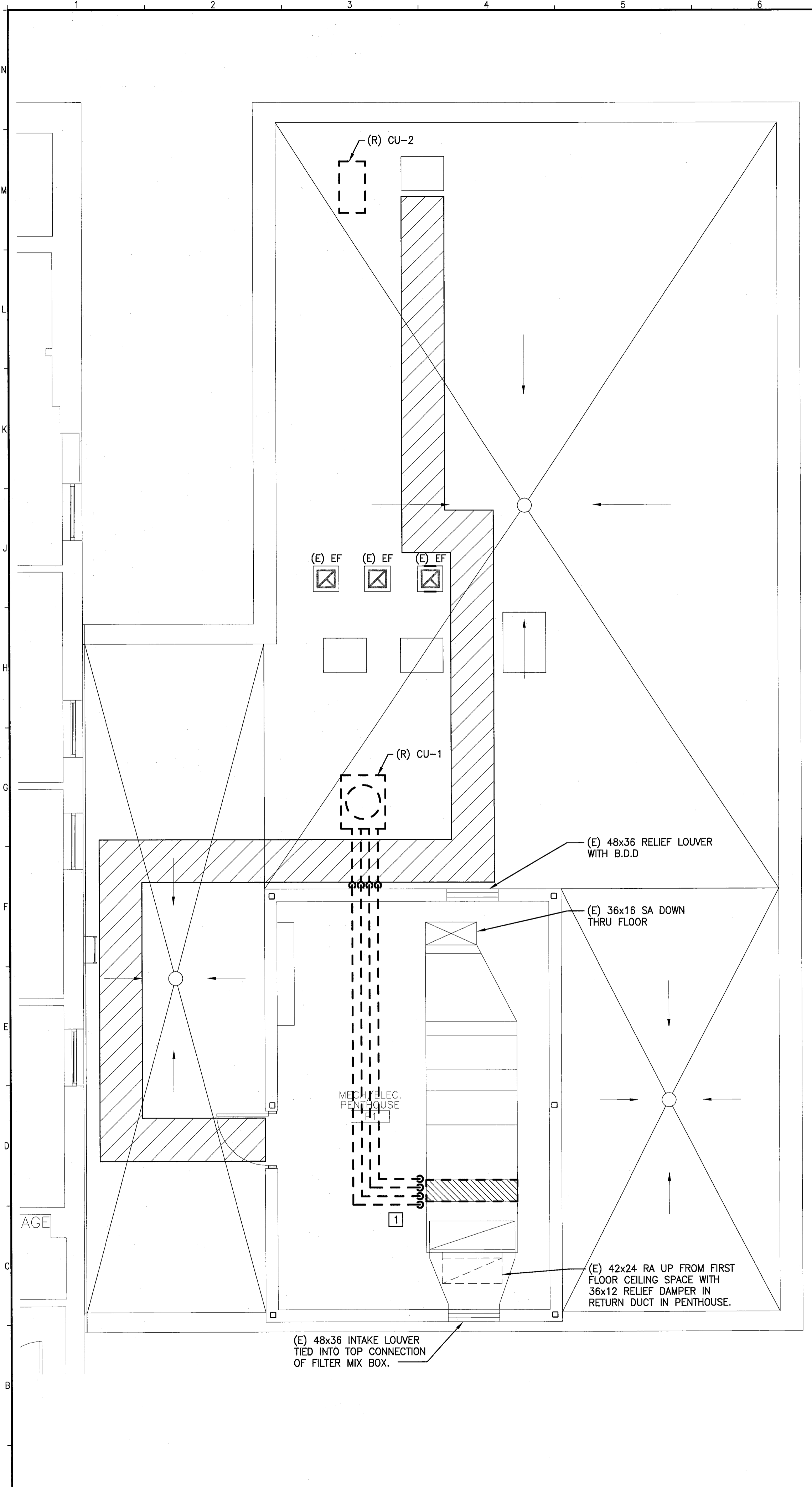
A1 DEMOLITION ROOF PLAN 1/4"=1'-0"
