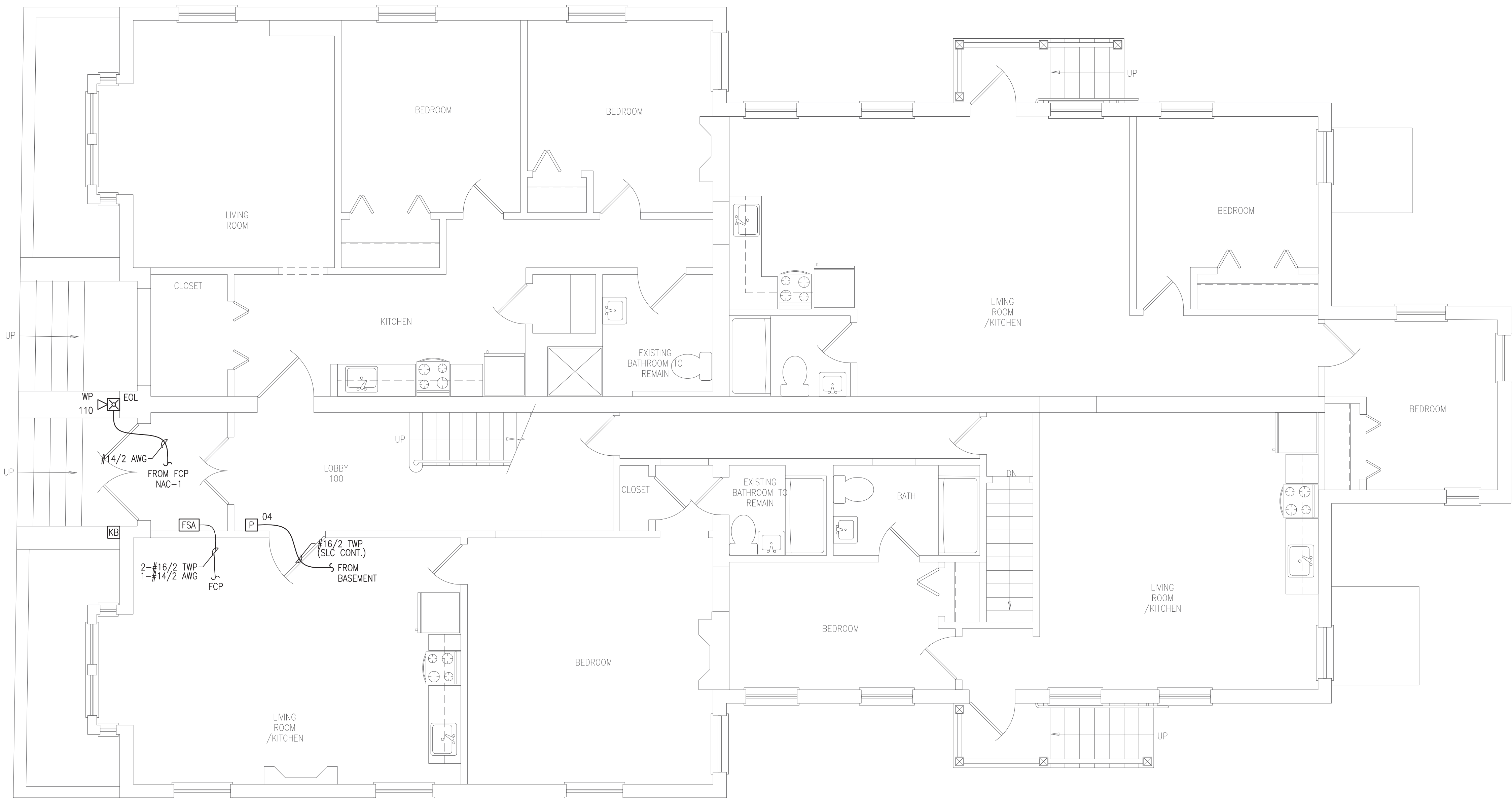
FIRST FLOOR FIRE ALARM PLAN SCALE: 1/4"=1'-0"
